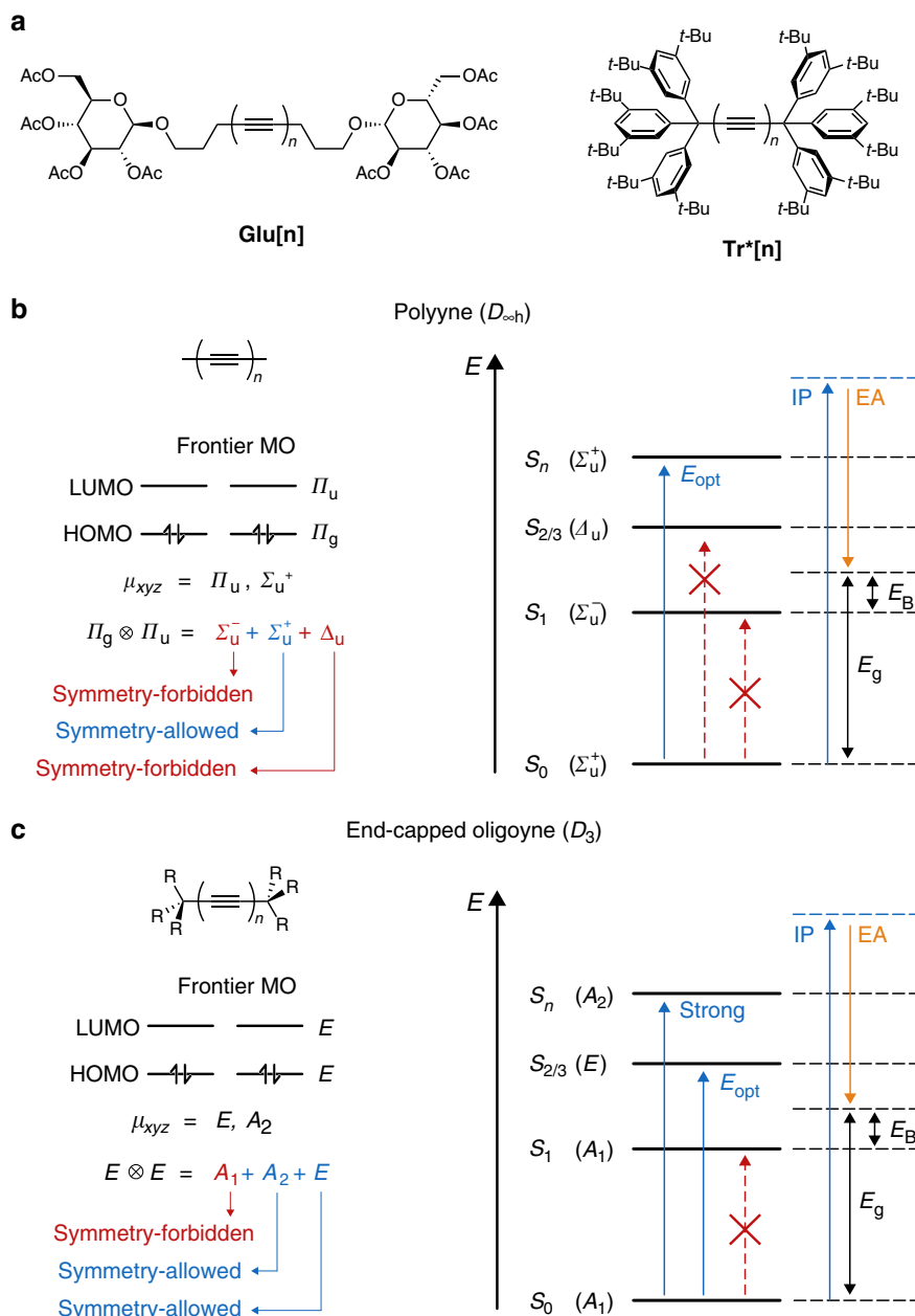
Fig. 1 Oligoynes and their optoelectronic properties. a Chemical structures of the C_2 -symmetric glycosylated oligoynes Glu [ n ], as well as the D_3 -symmetric oligoynes Tr *[ n ] featuring triarylmethyl endcapping groups. b, c Graphical representations of the symmetry arguments for the electronic transitions and their respective consequences for the optical gap E_{opt} and the fundamental gap E_g for b polyynes ( D_{\infty h} ) as well as c typical oligoynes R_3C-C \equiv C)_n-CR_3 (with the ionization potential IP , the electron affinity EA , the S_0 \rightarrow S_n transition (strong), and the electron-hole pair binding energy E_B ) 45 .
