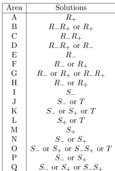
FIGURE 5.5. Candidate CRD solutions for two convex quadratic fluxes (case c < 0 ).
