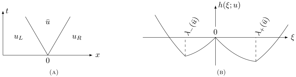
FIGURE 5.3. Structure of double-shock solutions
