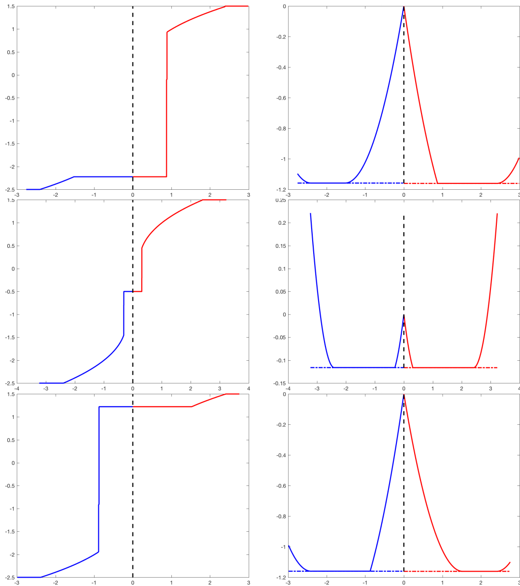
FIGURE 6.3. Three admissible solutions (from top to bottom). CRD solution u (left) and selection criterion h(\cdot; u) (right).
