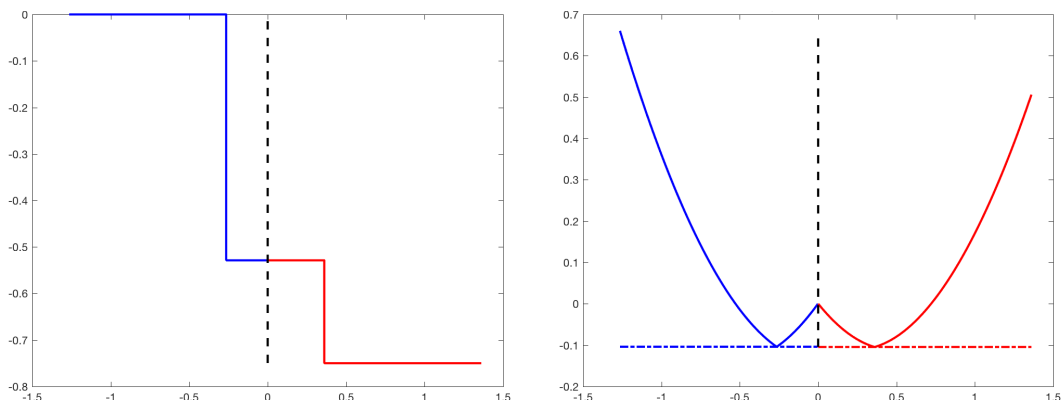
FIGURE 6.1. Numerical approximation of the double-shock solution. CRD solution u (left) and selection criterion h(\cdot; u) (right).
