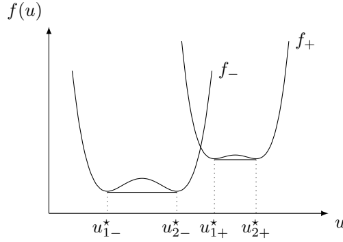
FIGURE 4.1. Standing shocks and non trivial inner solution
