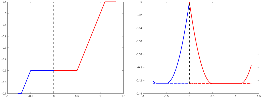
FIGURE 6.2. Numerical approximation of the double-rarefaction solution. CRD solution u (left) and selection criterion h(\cdot; u) (right).
