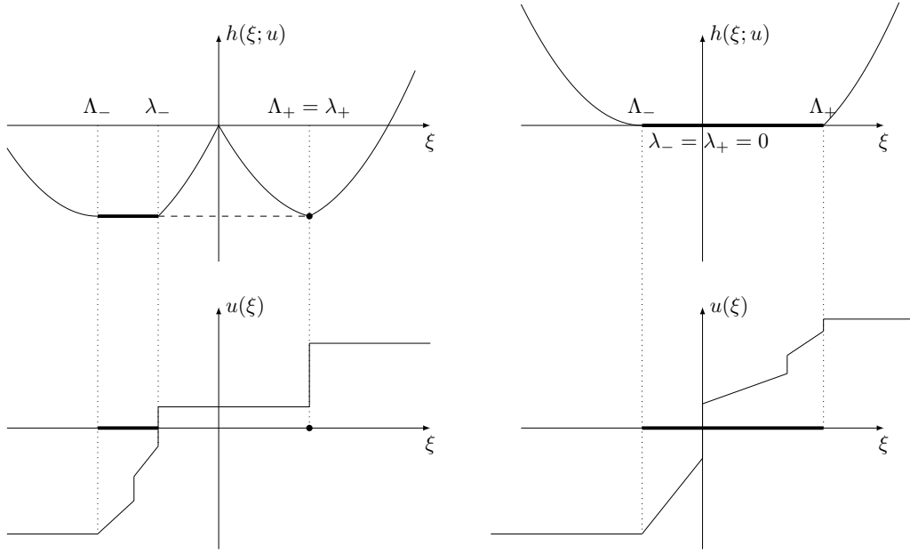
FIGURE 2.1. Illustration of case (ii) of the Corollary 2.2. The solution u is continuous at \xi = 0 (left) vs. discontinuous at \xi = 0 (right)
