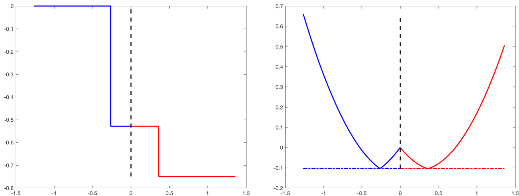
FIGURE 6.1. Numerical approximation of the double-shock solution. CRD solution u (left) and selection criterion h(\cdot; u) (right).
