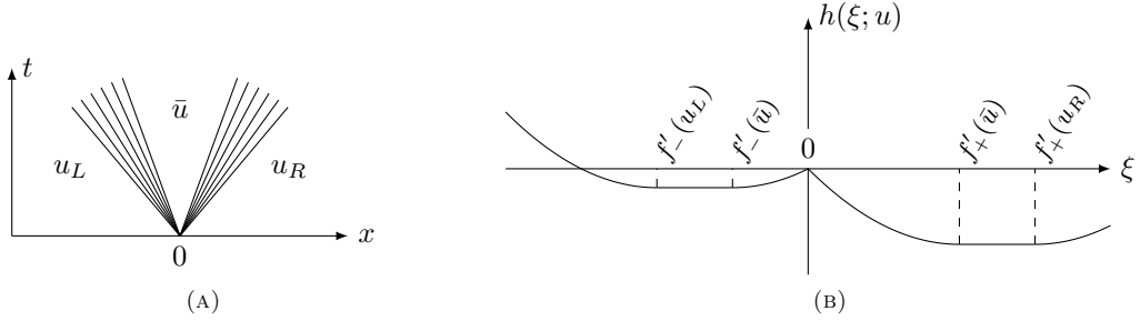
FIGURE 5.2. Structure of double-rarefaction solutions
