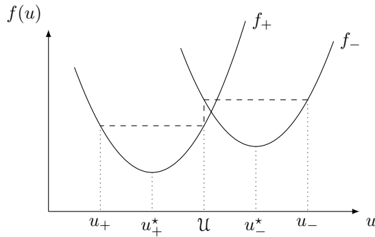
FIGURE 5.1. Non matching property
