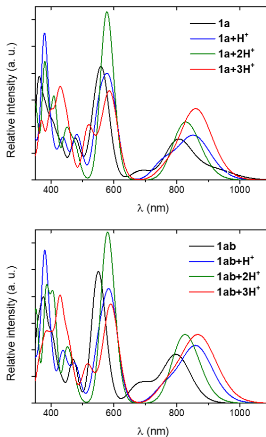
Figure 6. Theoretical absorption spectra of different protonation degrees of ACPs 1a (top) and 1ab (bottom) computed in DMSO. The spectra were obtained by convoluting the vertical TD-DFT spectrum with a Gaussian of FWHM = 0.3 eV.
