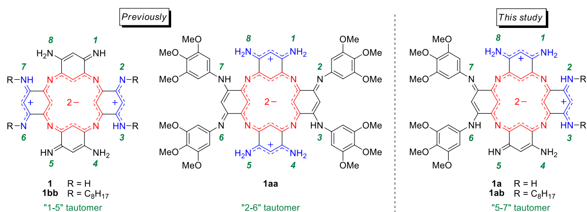
Figure 1. Scope of the previously synthesized and new azacalixphyrins (most stable tautomers). The two imine groups are at positions 1,5 for 1bb and 2,6 for 1aa , hence the displayed structures correspond to the "1-5" and "2-6" tautomers, respectively.
