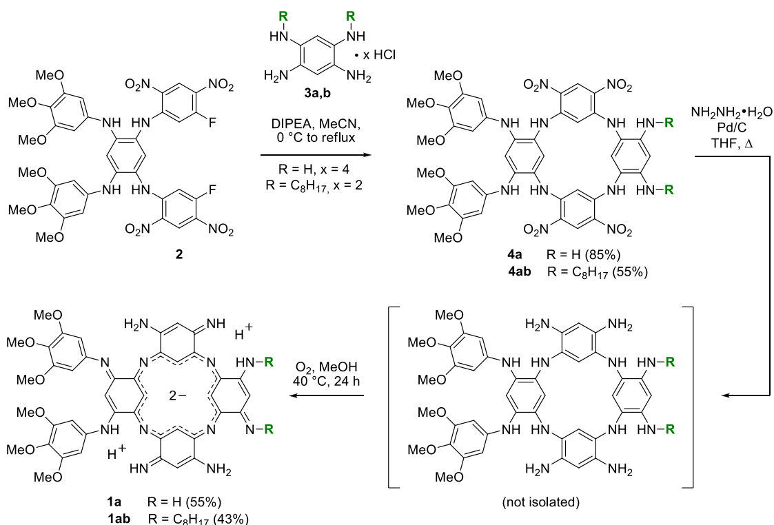
Scheme 1. Synthesis of azacalixpyrins 1a and 1ab .
