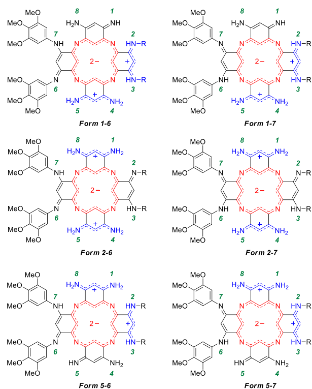
Figure 5. Selected most stable limit structures of azacalixpyrins 1a (R = H) and 1ab (R = C 8 H 17 ). Tautomers denomination depends on the position of the two imine functions.
