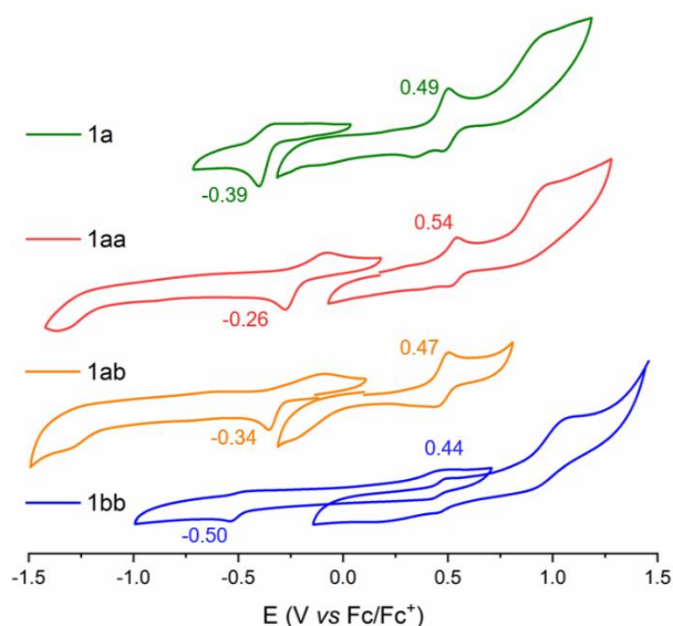
Figure 2. Cyclic voltammograms of ACPs in DMF solutions containing 0.1 M of [tBu 4 NPF 6 ].
