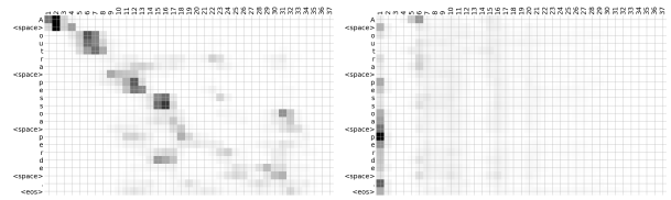
(a) wav2vec - entropy = 0.67 (b) fbanks - entropy = 0.81
