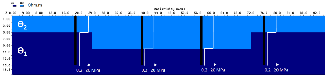
14 Figure 7: 2D section of subsoil displaying true ER distribution with boreholes positions in black and 15 associated tip resistance vertical profiles in white.
