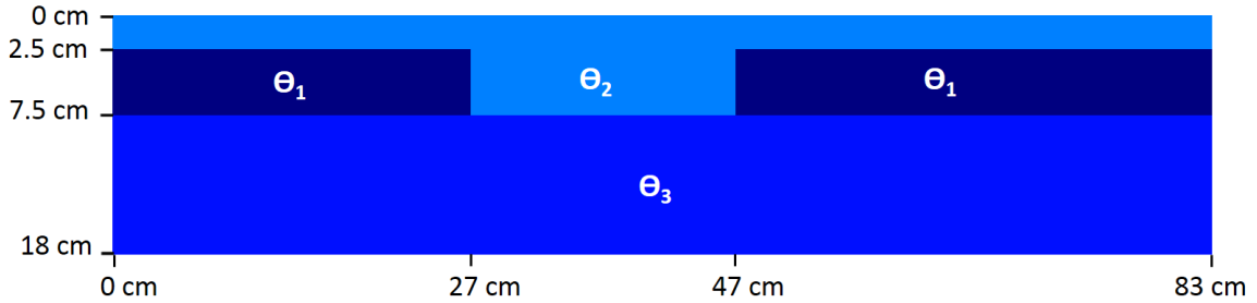
20 21 Figure 15: Scheme of the idealized section model (with vertical exaggeration), including the FoD constituent 22 events associated with the materials of the test bench
