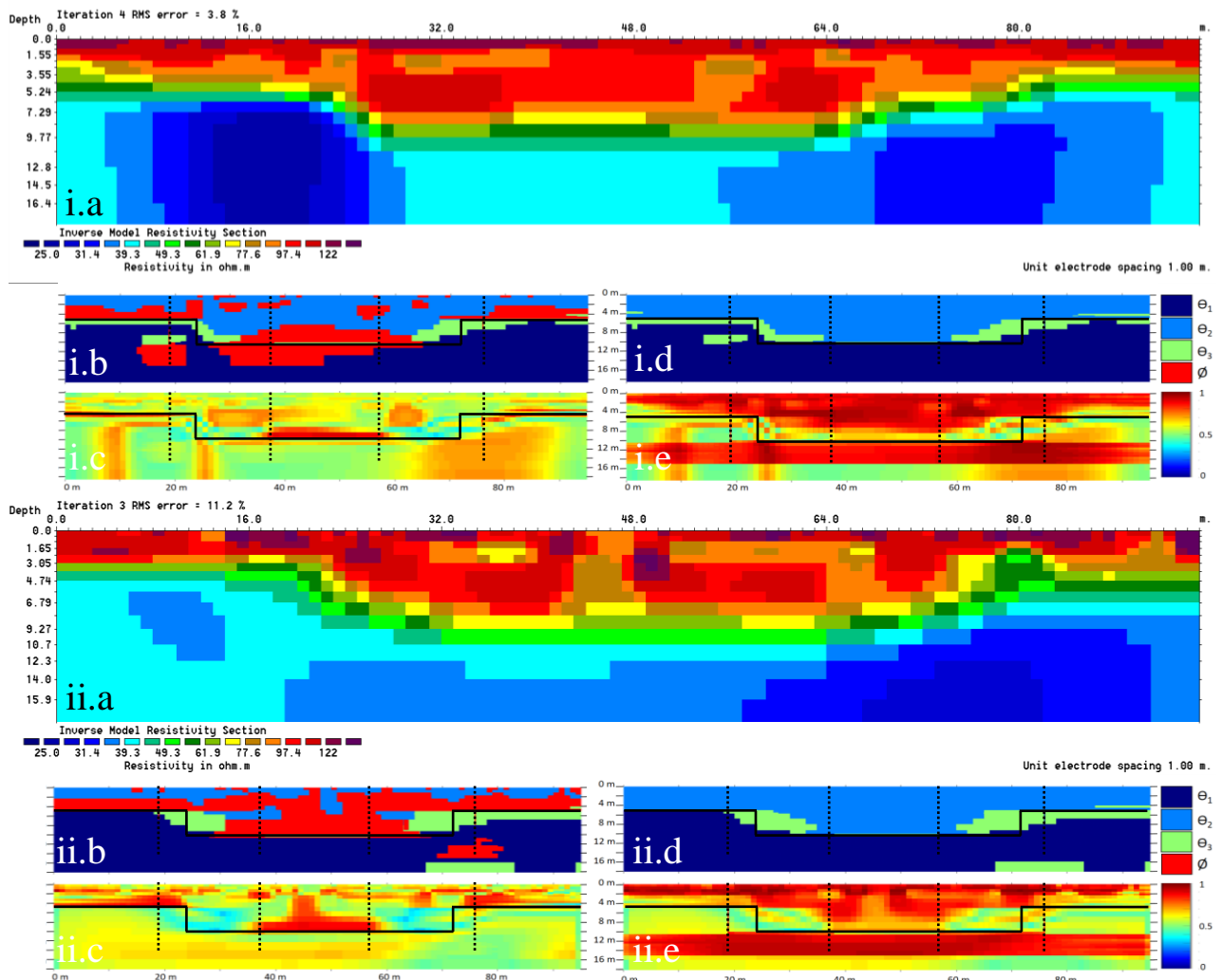
20 Figure 11: a) Subsoil section displaying inverted electrical resistivity values from i) 5% noise and ii) 15% 21 noise data acquisition. Representation of the events having the highest belief mass in b) and d) and their 22 associated mass values in c) and e). Figures on the left side are results for Smets fusion while figures on the 23 right side are results for PCR6 fusion. The sounding positions are in dashed lines while the black line 24 represent the position of the interface. 25
