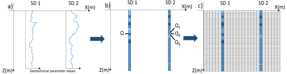
5 6 Figure 2: Construction of a geotechnical discretization mesh from two vertical boreholes acquisition (SD1 7 and SD2). a) Representation of the geotechnical values for SD1 and SD2 according to the depth. b) The 8 boreholes are divided in cells associated with belief mass equal to 1 for the considered event. c) Construction 9 of a new mesh according to the size and depth of the boreholes.
