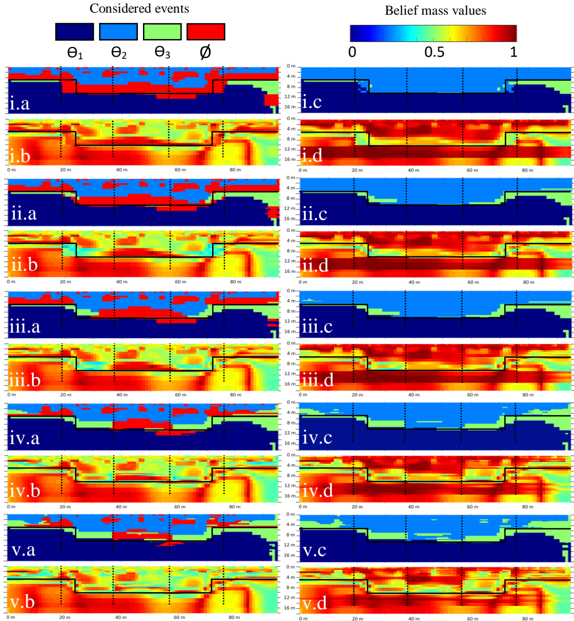
13 Figure 10: Representation of the events having the highest belief mass in a) and c) and their associated mass 14 values in b) and d), considering a 10% noise. In i) k=0.01 , ii) k=0.05 , iii) k=0.1 , iv) k=0.5 and v) k=1 .
