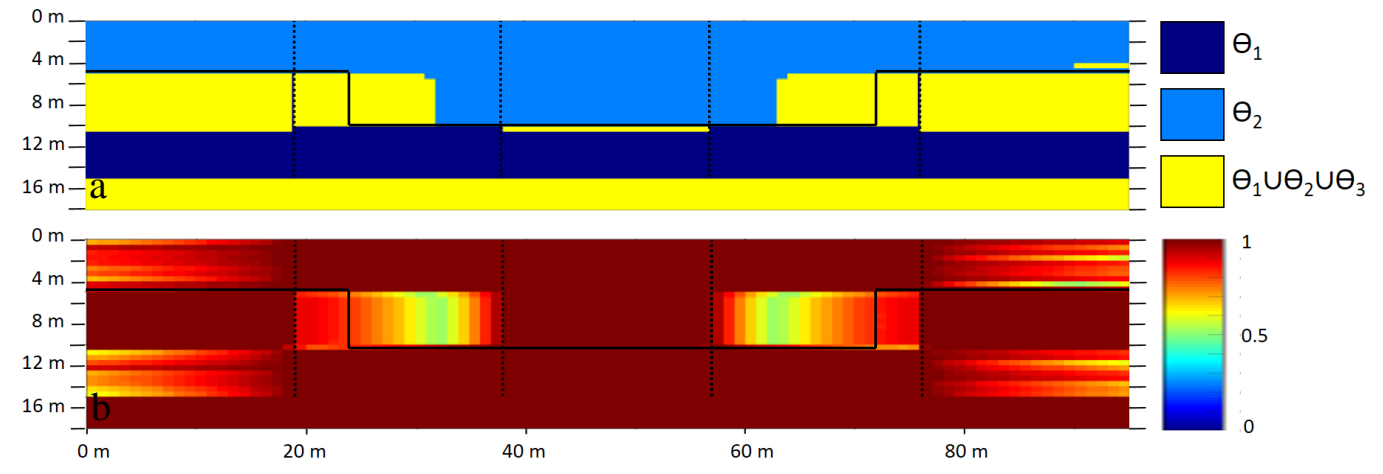
7 Figure 9: a) Representation of the events having the highest belief mass according to the BBA construction 8 from geotechnical data and b) the associated belief mass values. The borehole positions are in dashed lines 9 while the black line represent the position of the interface.
