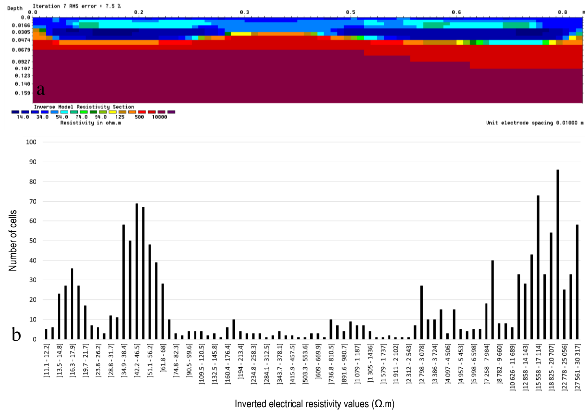
10 Figure 16: a) inverse model resistivity section obtained by roll along acquisitions in the central line of the 11 model and b) model classes' distribution of the cells presented in a), according to the electrical resistivity 12 values (Ω.m).
