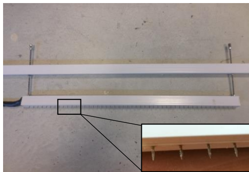
27 28 29 30 31 Figure 12: Mini ERT device with 48 electrodes spaced 1 cm, adjustable height, used for electrical 32 acquisitions in the test bench.
