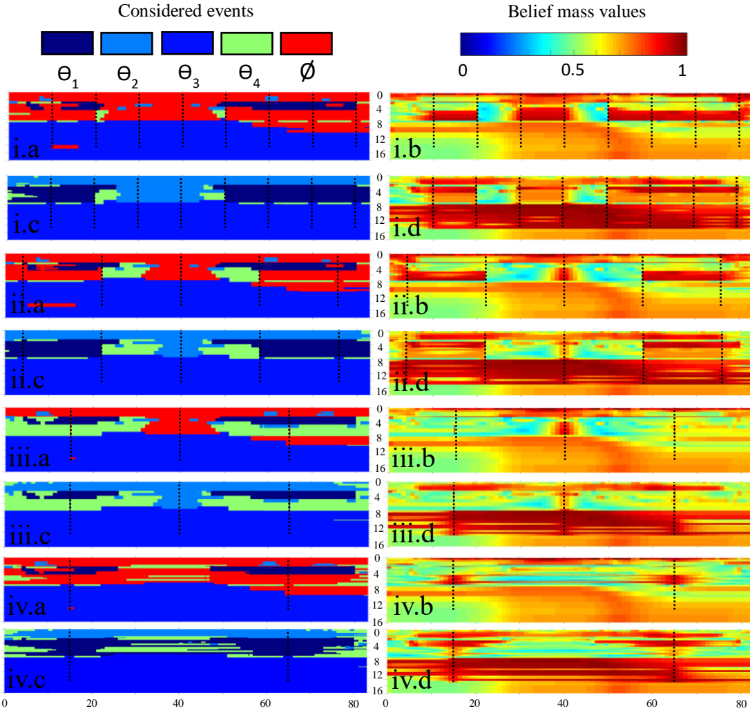
2 Figure 17: Representation of the events having the highest belief mass in a) and c) and their associated mass 3 values in b) and d). For i) 8 boreholes, ii) 5 boreholes, iii) 3 boreholes, iv) 2 boreholes are considered. For 4 each case, (a,b) figures are results of Smets fusion, while (c,d) figures are results of PCR6 fusion. The 5 borehole positions are in dashed lines.
