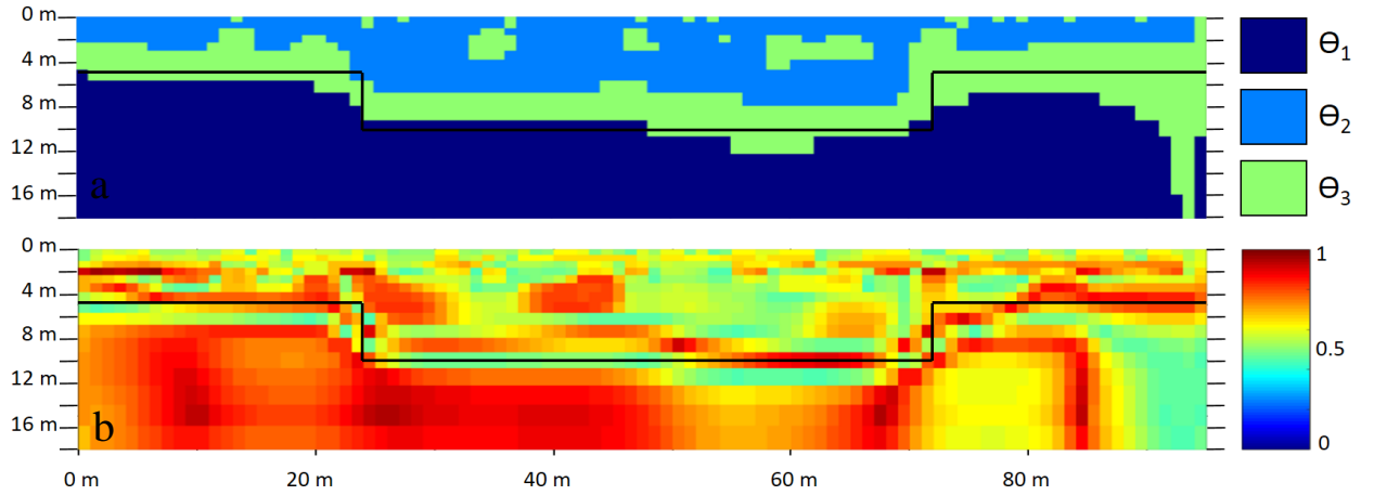
2 Figure 6: a) Representation of the event having the highest belief mass according to the BBA construction 3 from geophysical data and b) the associated belief mass values, considering a 10% noise. The black line 4 represent the position of the interface.
