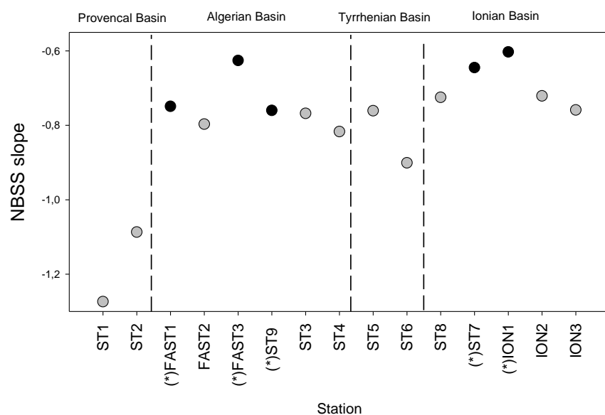
Figure 8: NBSS slope for all stations during PEACETIME survey.
