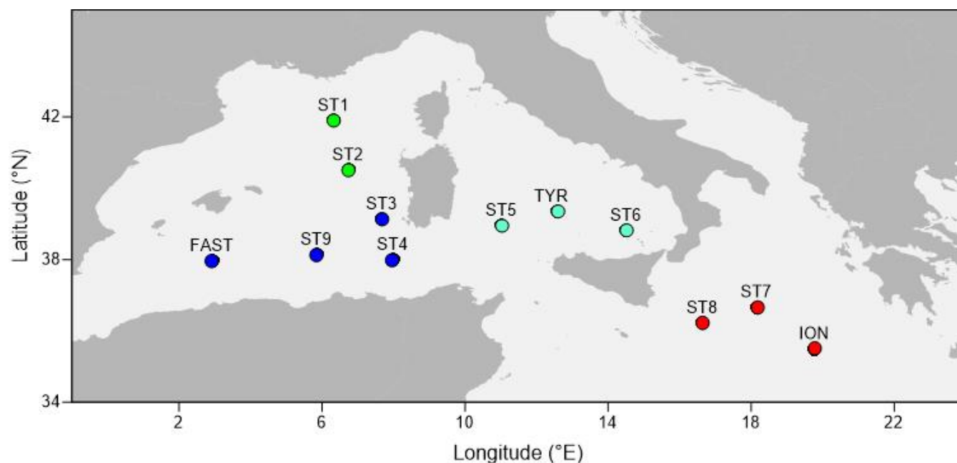
Figure 1: Map with the sampling points during PEACETIME cruise 2017. The colours of the points indicate the different regions considered in the course of the study. Green dots: Provencal basin (PB); Dark blue dots: Algerian Basin (AB); Light blue dots: Tyrrhenian Sea (TB); Red dots: Ionians Basin (IB).
