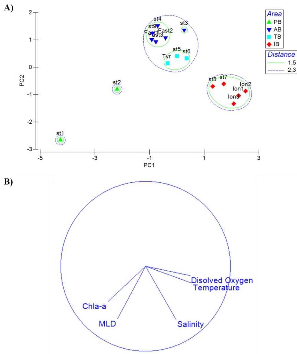
Figure 3: Principal Component Analysis (PCA) ordination of five environmental indicators: Mixed/layer Depth (MLD), Integrated values of Chl-a concentration, mean values on the upper 0/300 m of temperature, salinity and dissolved oxygen. (A) Plots of the stations and (B) variables on the first factorial plan. AB: Algerian Basin, PB: Provencal Basin, TB: Tyrrhenian Basin, IB: Ionian Basin.
