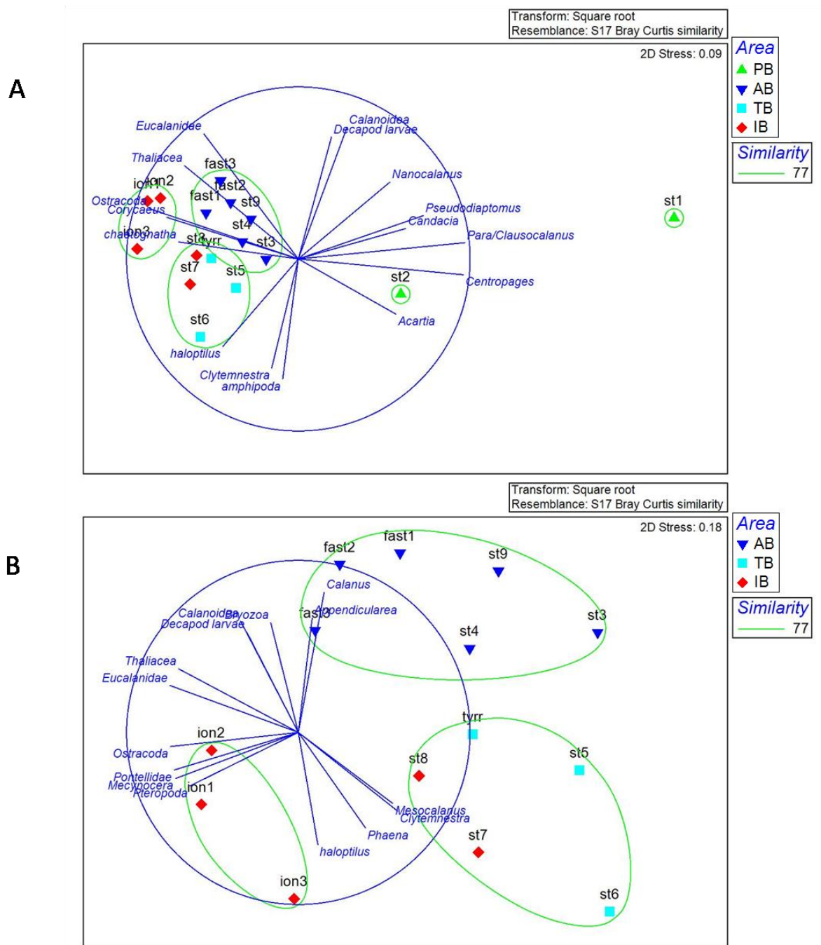
Figure 6: NMDS analysis of the zooplankton taxa for the whole stations (A) and with exclusion of st 1 and st2 (B): plot of the stations and the taxa correlated at >0.65 with the axes. Colour of the stations represents the eco-regions identified by the PCA on the environmental analysis (see Fig. 2). This analysis was performed on the zooplankton collected with the data from N 200 . PB: Provencal Basin, AB= Algerian Basin, TB =Tyrrhenian Basin, IB = Ionian Basin.
