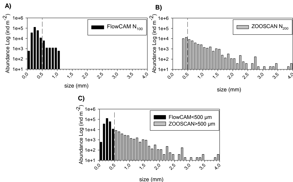
Figure 2: Size spectrum of ST ION1 as an example obtained by: A) FlowCAM (N 100 ), B) ZOOSCAN (N 200 ) and C) combination of FlowCAM (N 100 counting only zooplankton smaller than 500 µm of ESD) and ZOOSCAN (N 200 counting only zooplankton bigger than 500 µm of ESD)
