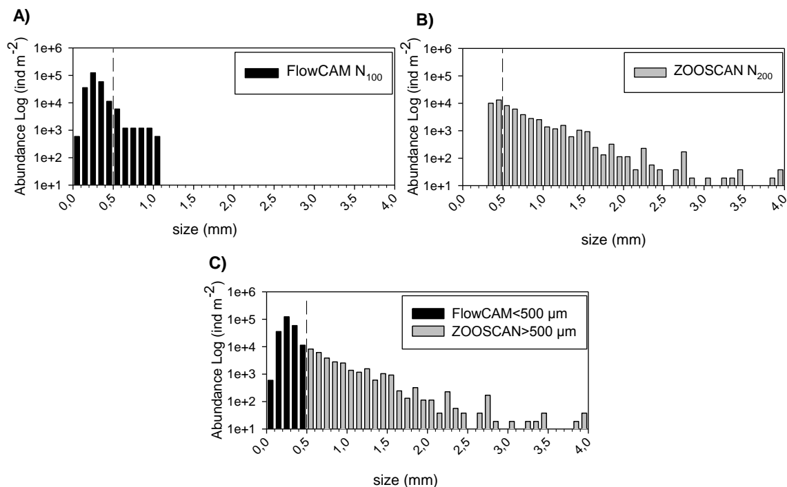
Figure 2: Size spectrum of ST ION1 as an example obtained by: A) FlowCAM (N 100 ), B) ZOOSCAN (N 200 ) and C) combination of FlowCAM (N 100 counting only zooplankton smaller than 500 μm of ESD) and ZOOSCAN (N 200 counting only zooplankton bigger than 500 μm of ESD)
