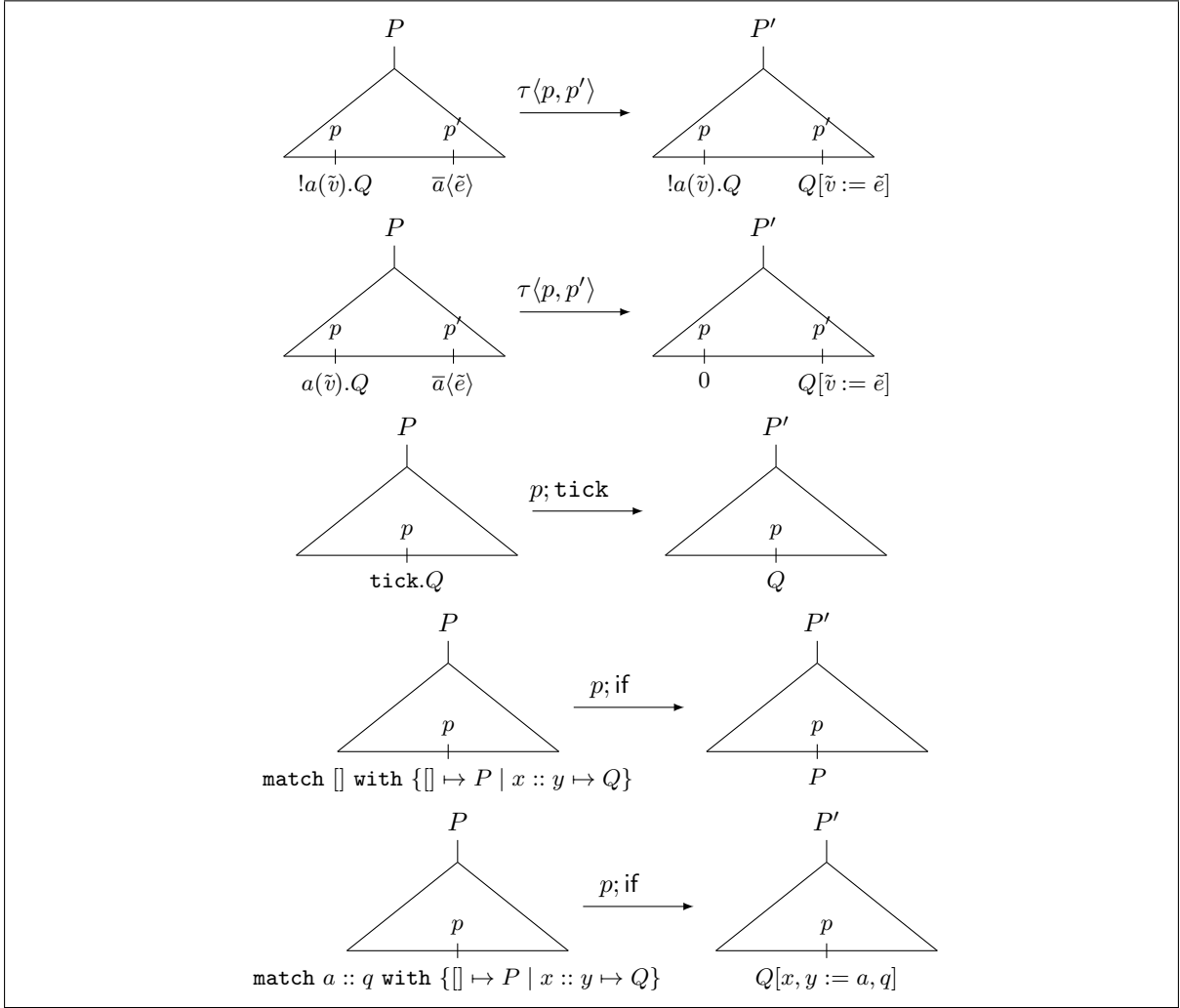
Figure 16: Semantics for Causal Complexity
