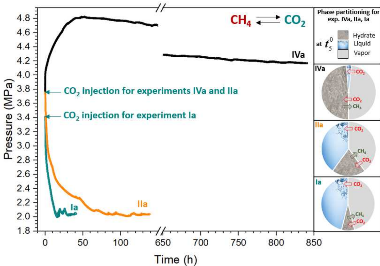
Figure 6: Pressure evolution with time during CH 4 -CO 2 exchange experiments (stirring off) starting from three distinct CH 4 hydrates systems formed with different driving forces (exp. Ia vs IIa) or experimental pathways (exp. Ia vs IIa).
