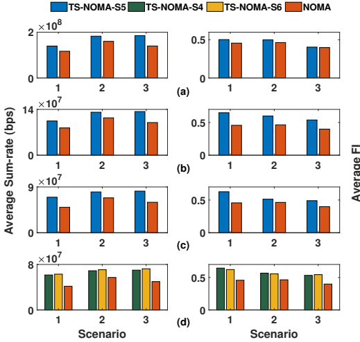
Fig. 2: Comparison of sum-rate and FI for TS-NOMA and NOMA for the case of no dimming ( \delta = 1 ).
