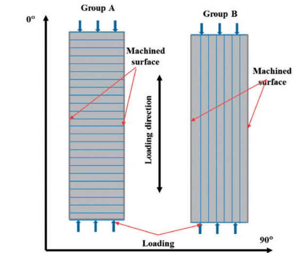
Figure 2. Schema of loading direction during compression test in group A and group B specimens.
