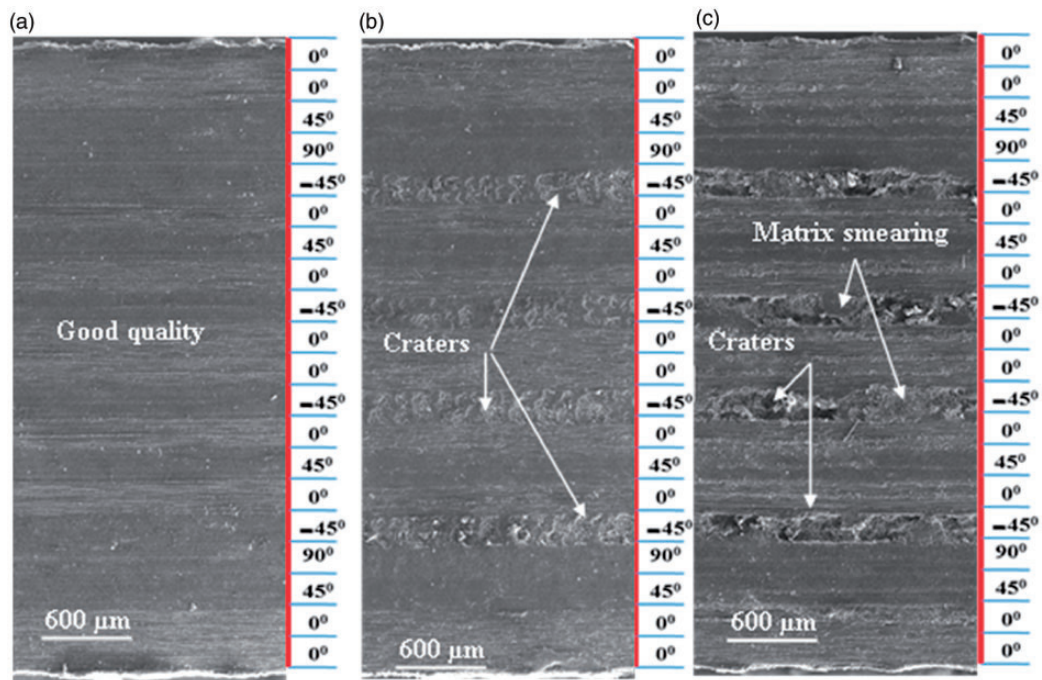
Figure 9. SEM images of machined surface for specimens of group B (a) good quality with V_c = 150\ \text{m/min} , V_f = 500\ \text{mm/min} , and L_c = 0.28\ \text{m} , (b) medium quality with V_c = 150\ \text{m/min} , V_f = 1500\ \text{mm/min} , and L_c = 1.68\ \text{m} , and (c) poor quality with V_c = 339\ \text{m/min} , V_f = 29\ \text{mm/min} , and L_c = 0.28\ \text{m} .
