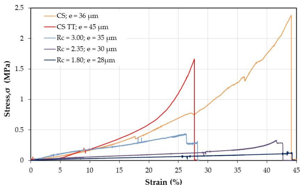
Figure 11. Effect of thermal treatment on mechanical response of chitosan and PEC films in the wet state after stabilization in PBS at pH = 7.4.
