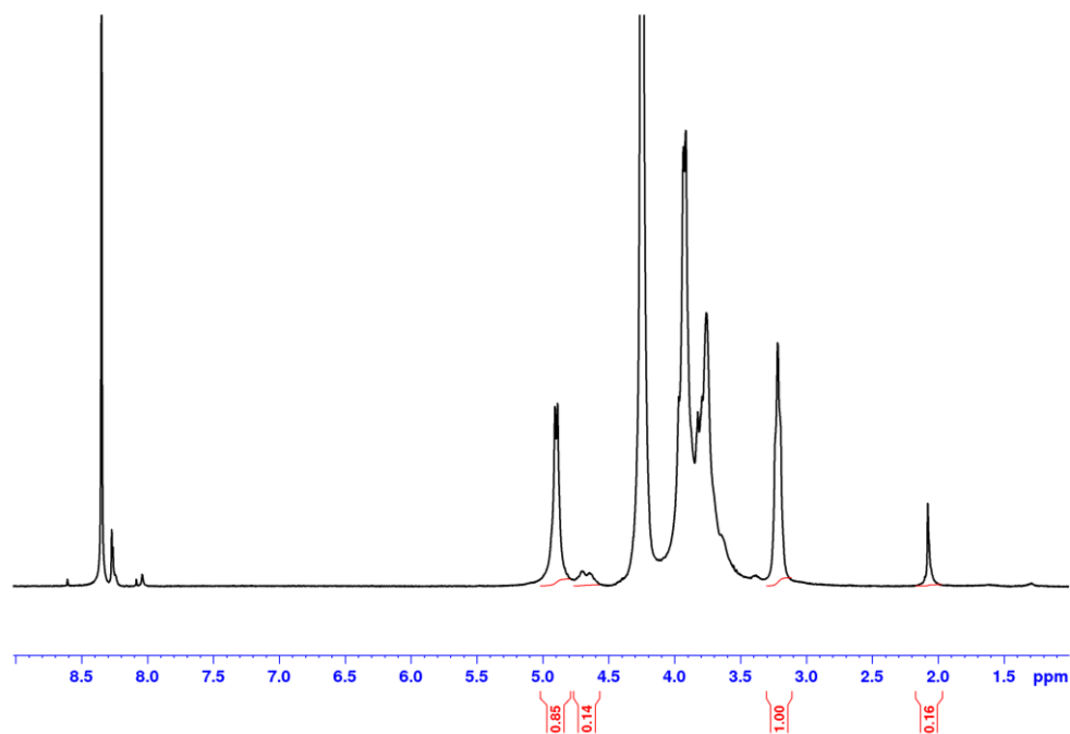
Figure 6. ^1\text{H} NMR spectrum obtained on a chitosan film casted from chitosan in \text{D}_2\text{O}/\text{DCl} solvent at 85^\circ\text{C} .
