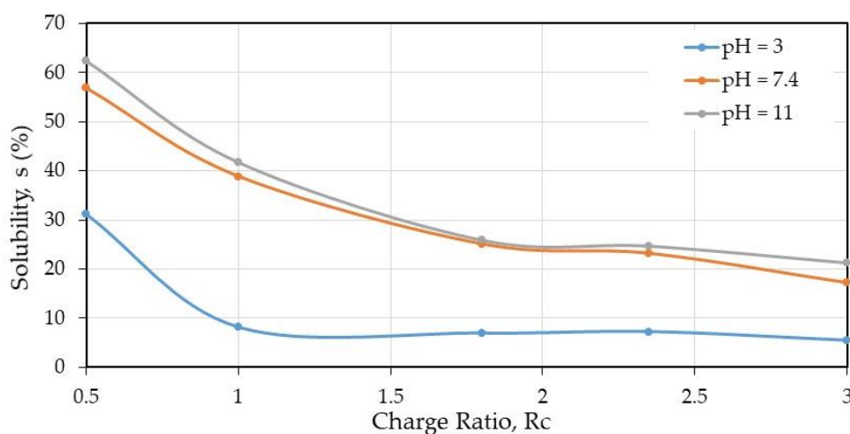
Figure 5. Partial solubility (%) at different pH on PEC films prepared in W/FA 50/50 v/v as a function of charge ratio.
