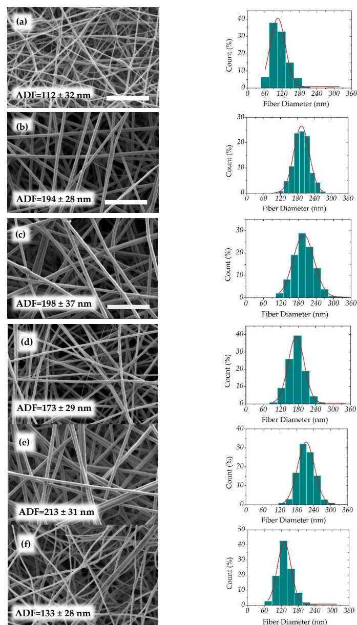
Figure 13. Scanning electron microscopy images of nanofibers obtained at different charge ratios and corresponding average fiber diameters (AFD) (nm) together with their diameter distribution. (a) R_c = 0.5 , (b) R_c = 1.0 , (c) R_c = 1.8 , (d) R_c = 2.35 , (e) R_c = 3.0 , and (f) CS. Scale bar = 3 \mu\text{m} .
