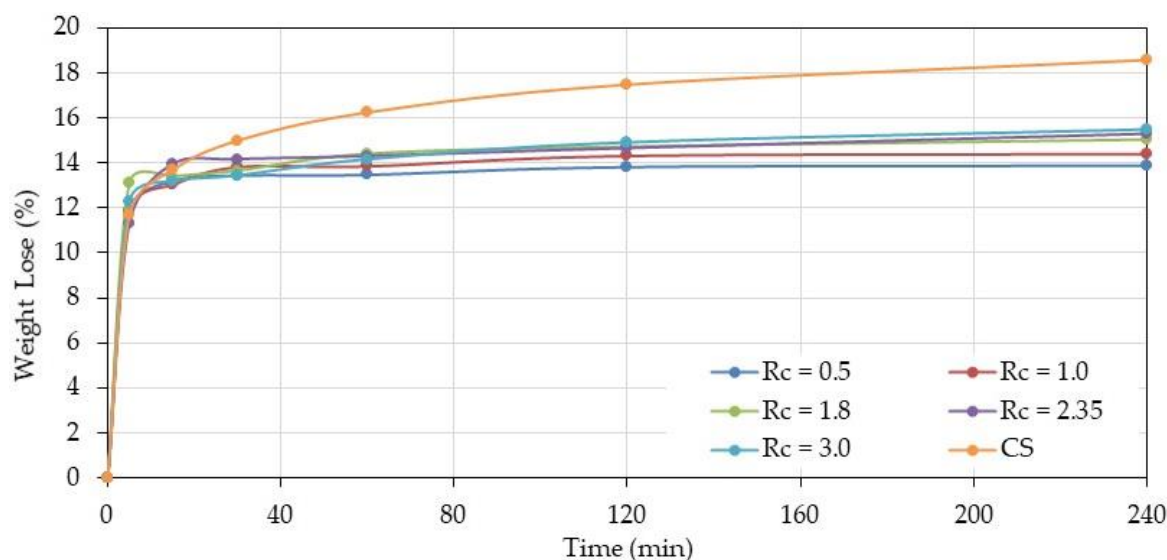
Figure 1. Weight loss of polyelectrolyte complex (PEC) at different chitosan (CS)/hyaluronan (HA) charge ratios R_c compared with pure chitosan (CS) prepared in water (W)/formic acid (FA) (50/50 v/v ) as a function of time at 120 °C.
