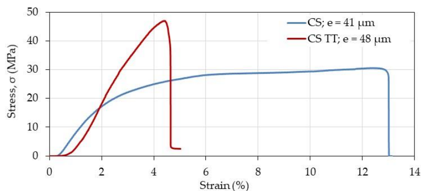
Figure 9. Effect of thermal treatment (TT) on mechanical chitosan film response in the dried state. The thickness ( e ) of the film samples was found around 40–50 \mu\text{m} .
