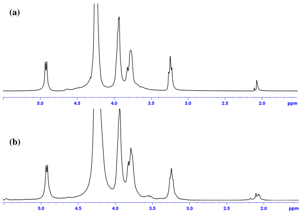
Figure 7. Influence of thermal treatment on ^1\text{H} NMR spectrum for film of chitosan obtained after chitosan solubilization in HCl in absence of thermal treatment (a); and after thermal treatment (b). Solvent \text{D}_2\text{O}/\text{DCI} at 85^\circ\text{C} .
