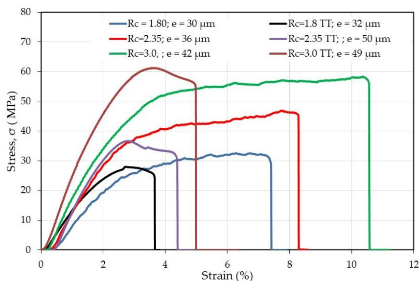
Figure 10. Effect of thermal treatment (TT) on mechanical response of PEC films in the dried state. Stress as a function of strain (%) before and after thermal treatment for different complexes characterized by R_c .
