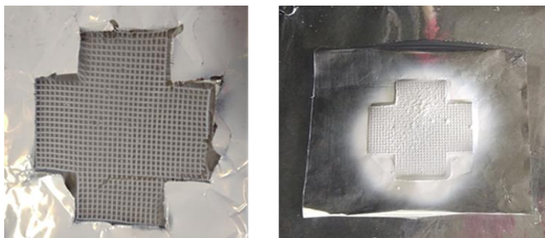
Figure 12. CS/HA+ polyethylene oxide (PEO) nanofibers on metallic collectors utilized for the electrospinning process.
