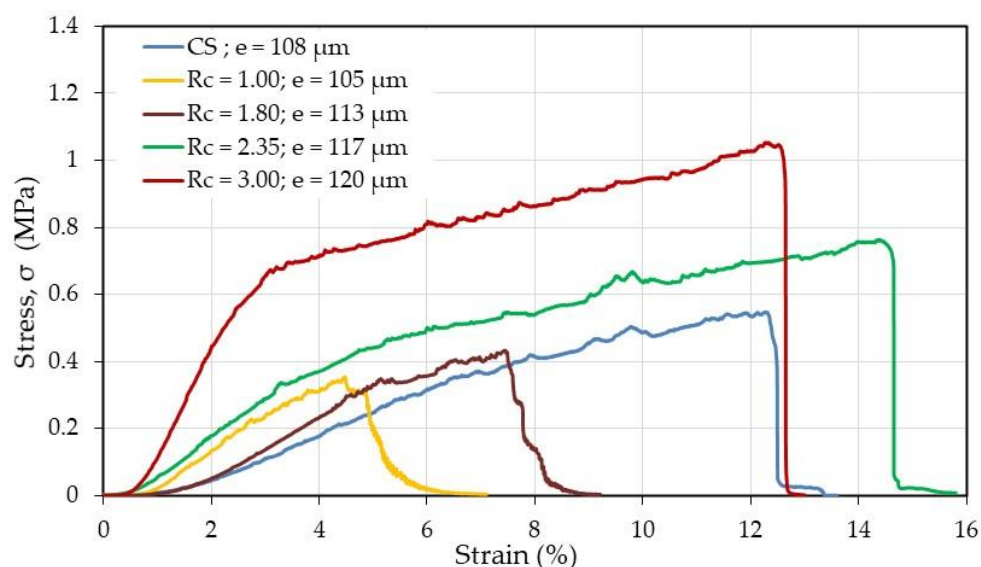
Figure 14. Mechanical behavior of chitosan and as-spun PEC fiber samples in dried state.
