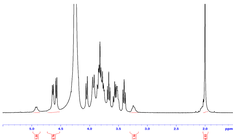
Figure 8. ^1\text{H} NMR spectrum of a complex film prepared at a charge ratio R_c = 0.5 formed in W/FA (50/50 v/v ) after thermal treatment. Solvent \text{D}_2\text{O}/\text{DCI} at 85^\circ\text{C} .
