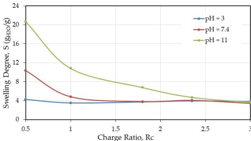
Figure 4. Swelling degree (g water/g dried material) as a function of the charge ratio after thermal treatment.
