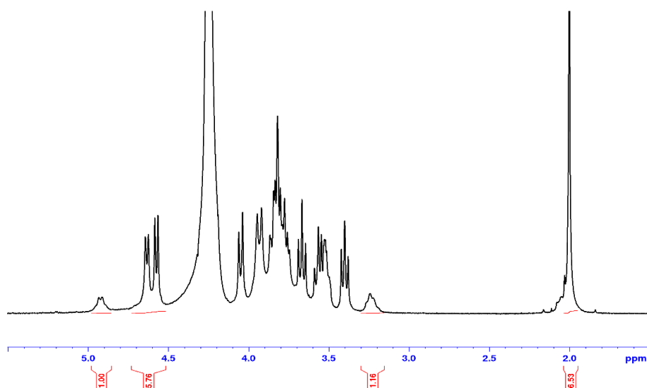
Figure 8. ^1\text{H} NMR spectrum of a complex film prepared at a charge ratio R_c = 0.5 formed in W/FA (50/50 v/v ) after thermal treatment. Solvent \text{D}_2\text{O}/\text{DCl} at 85^\circ\text{C} .
