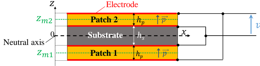
Figure 4: Beam layers and electrodes connection in parallel
