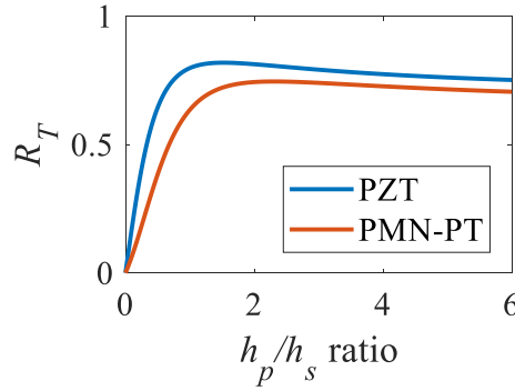
Figure 8: \mathcal{R}_T as a function of the thickness ratio for PZT or PMN-PT patches and steel substrate ( Y_s = 200 GPa). Plane stress assumption and piezoelectric coefficients of Table 1 are considered.
