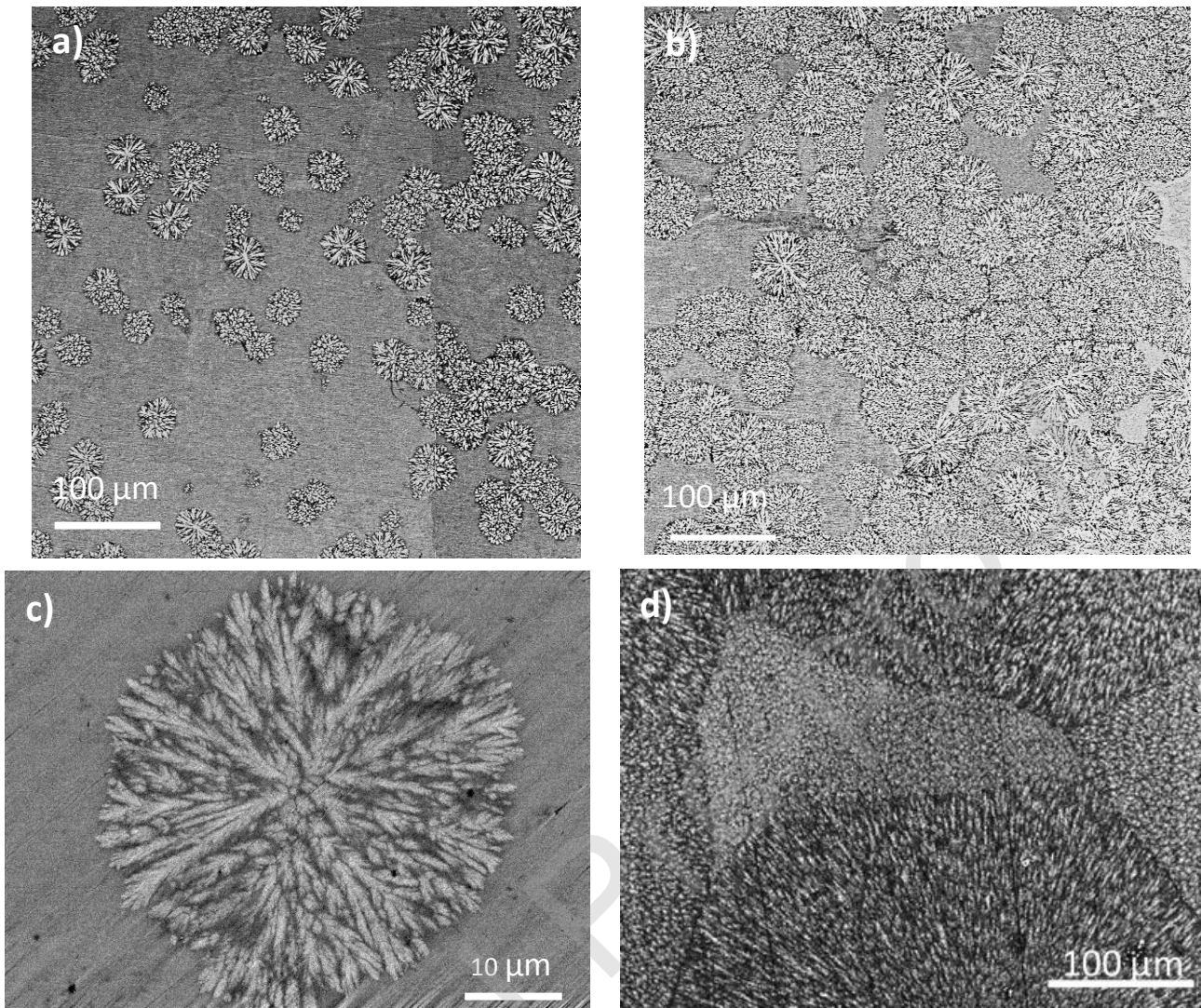
Fig. 9: Microstructures of the glass ceramics: SEM observations of a) the B_2S_3\_N\_C2h-1 grade ( C_f=22\% ) and b) the B_2S_3\_N\_C2h-2 grade ( C_f=49\% ); c) High magnification SEM images of a spherulite in the B_2S_3\_C4h grade, and d) the almost fully crystallized B_2S_3\_C1w grade.
