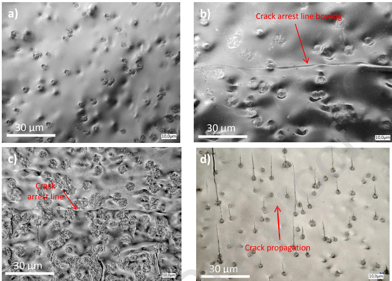
Fig. 10: Optical microscopy images of the fracture surface of SEPB specimens with \approx 5 (a,b,d) and \approx 49 (c) vol.% crystallized phase. a) craters and bumps left on the crack path due to the by-passing of the spherulites; crack front bowing at particle sites in b) B_2S_3\_N\_C30m and c) B_2S_3\_N\_C2h-2 . The final fast fracture stage induces some local microcracks at the particles pointing toward the crack propagation direction (d) .
