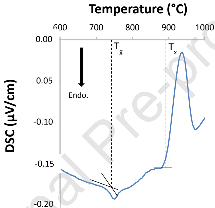
Fig. 2: DSC signal at 10\text{ }^\circ\text{C}/\text{min} for glass grains (50 mg with a granulometry comprised between 100 and 200 \mu\text{m} ). The black lines represent asymptotes of the different foot peaks. The black dotted lines are placed at the intersections of the asymptotes; they represent T_g and T_x .
