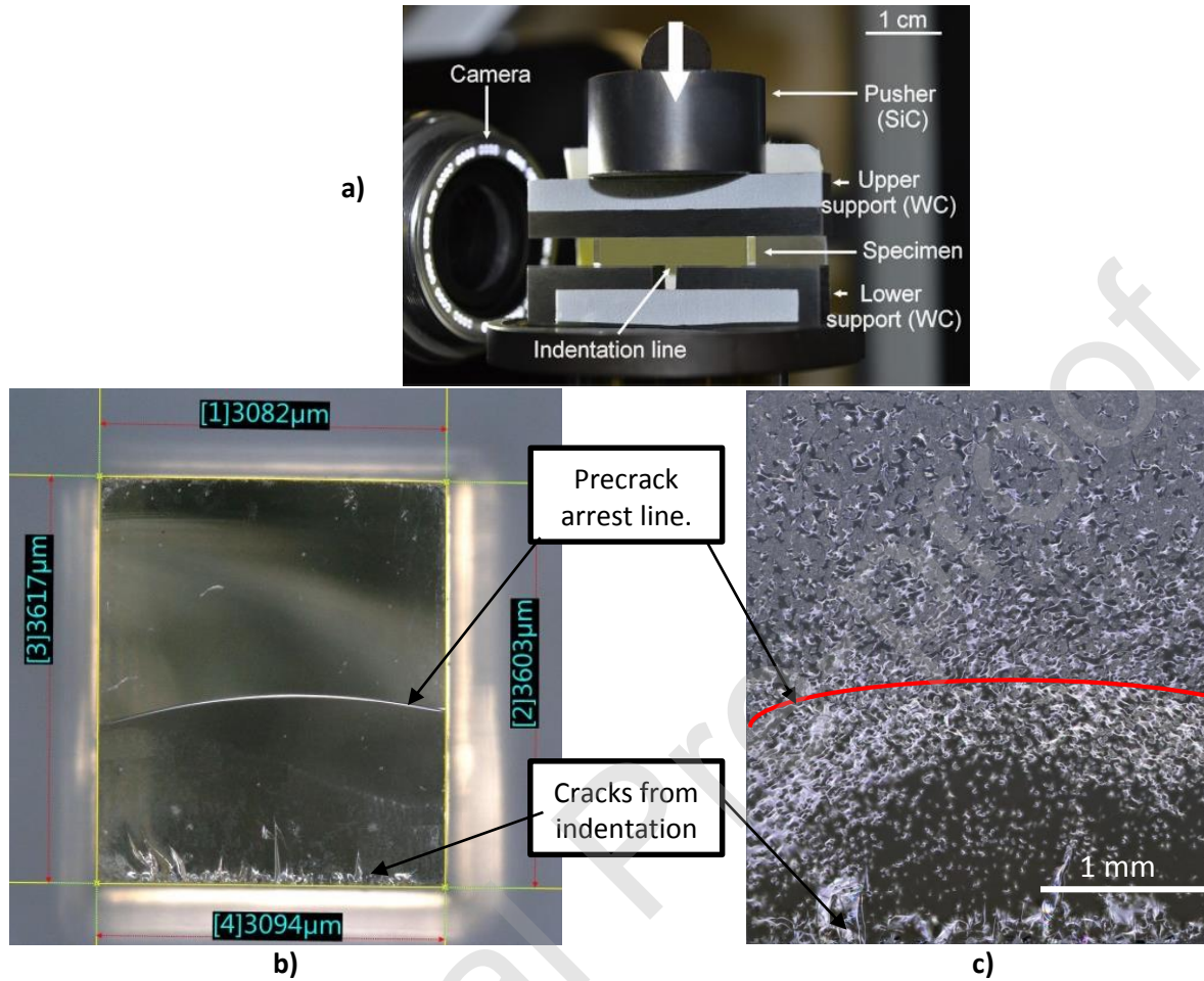
Fig. 1: Pictures of a SEPB testing specimens. a) \text{B}_2\text{S}_3 during the precracking step, b) \text{B}_2\text{S}_3 after the three-point bending fracture and c) fractured surface of the \text{B}_2\text{S}_3\text{-N-C2h-1} after the SEPB procedure.
