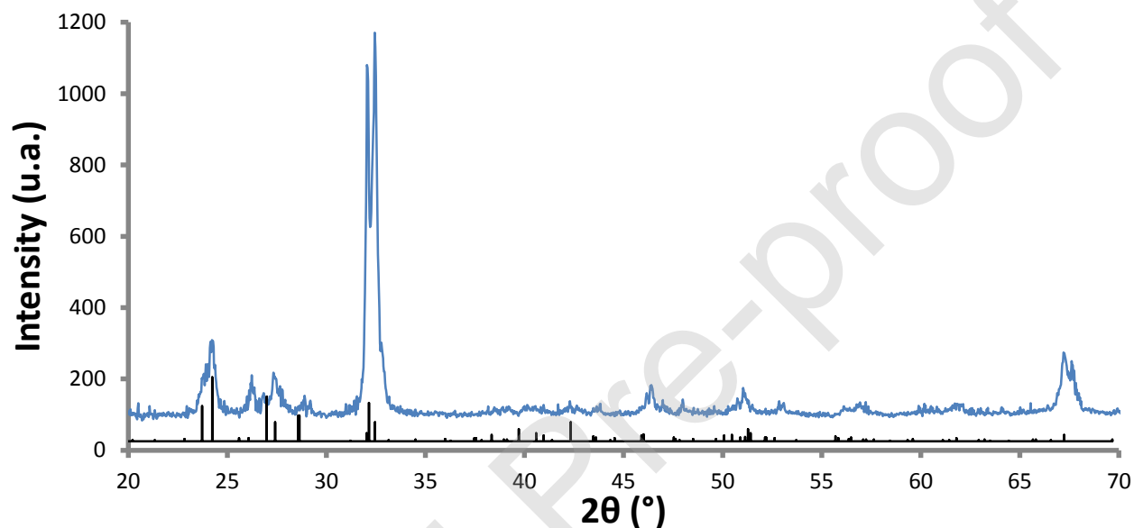
Fig. 7: Diffraction pattern of the GC after a heat treatment of 72 h at 825 °C (blue curve). For comparison, the diffract pattern of Ba 2 Si 3 O 8 (00-027-1035) is also reported in black.
