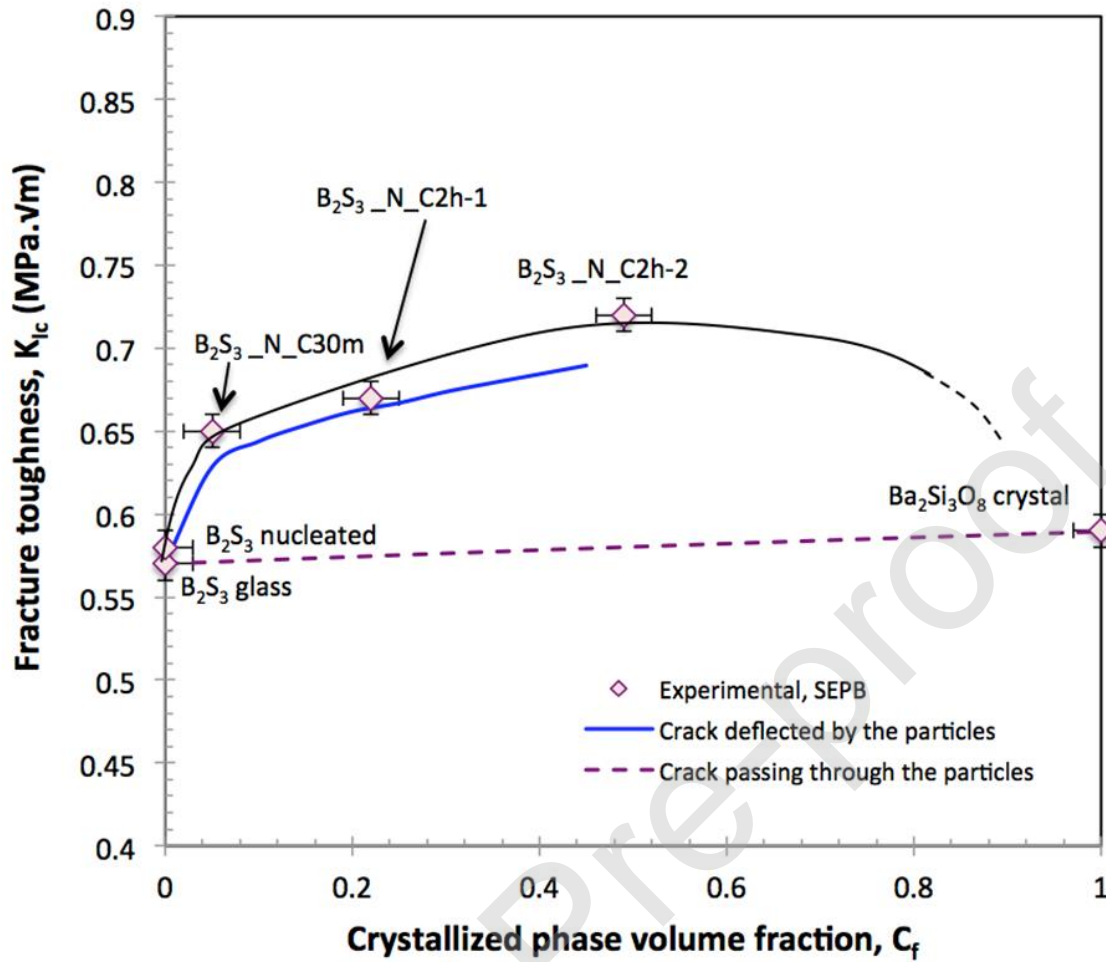
Fig. 11: Toughness of the sample determined by SEPB. The dotted line represents a guide for the eyes.
