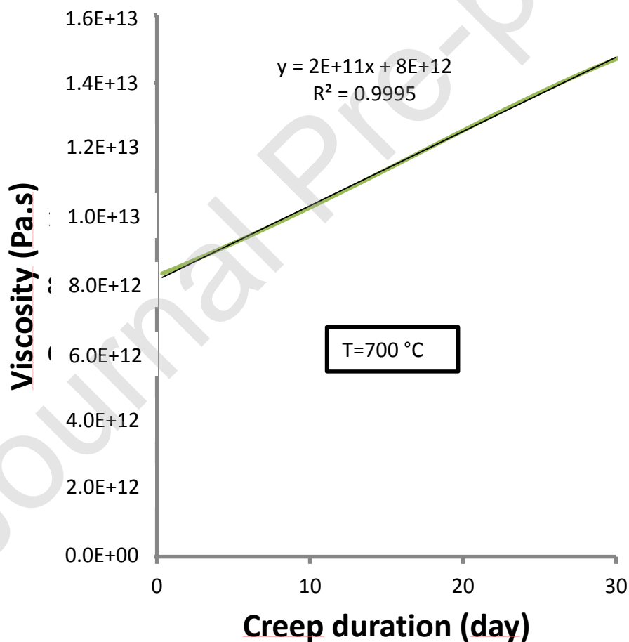
Fig. 12: Evolution of glass viscosity in function of creep duration at 700 °C.
