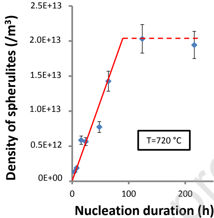
Fig. 3: a) Nuclei density as a function of the heat-treatment temperature; b) Nuclei density as a function of the nucleation treatment duration at 720 °C. The red plain and dotted lines represent the linear evolution and the hypothesized saturation plateau of the nuclei density respectively.
