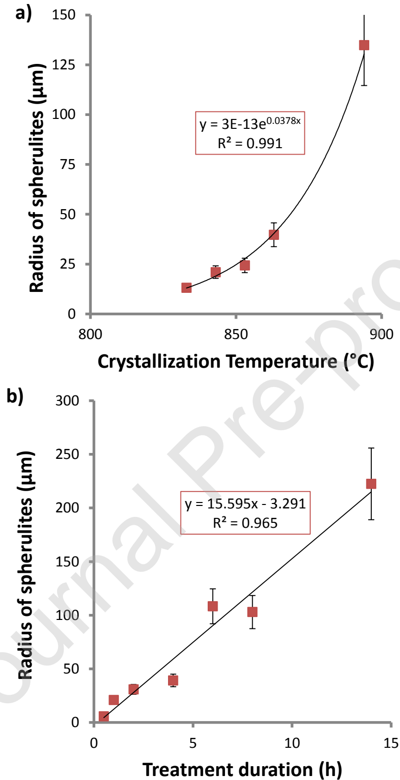
Fig. 6: a) Temperature dependence of the mean radius of the spherulite crystals for a thermal treatment of 1 h between 820 and 900 ^{\circ}\text{C} ; b) Evolution of the mean spherulite radius with time at 825 ^{\circ}\text{C} .
