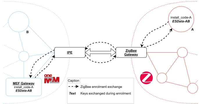
Fig. 2. Enrolment of a ZigBee node with our MEF gateway
