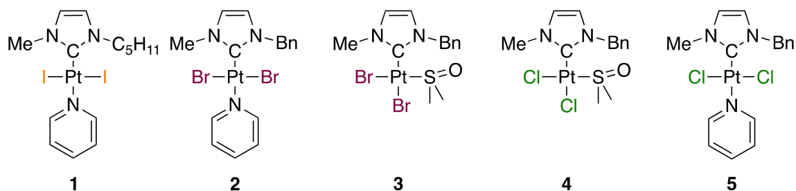
Scheme 2. Molecular structure of the N -heterocyclic carbene (NHC)-Pt(II) references.
