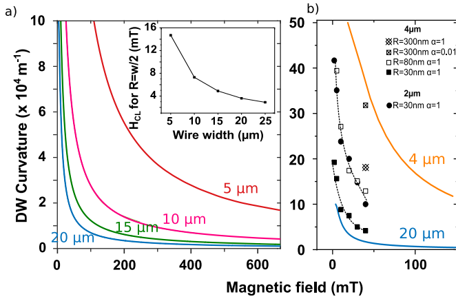
FIG. 5. (a) Calculated H_{CL} profile for \sigma_E=1.01 \times 10^{-2} N/m (CoFeB) for different wire widths. H_{CL} values corresponding to R=w/2 as a function of the wire width (inset). (b) Comparison with micromagnetic simulations.
