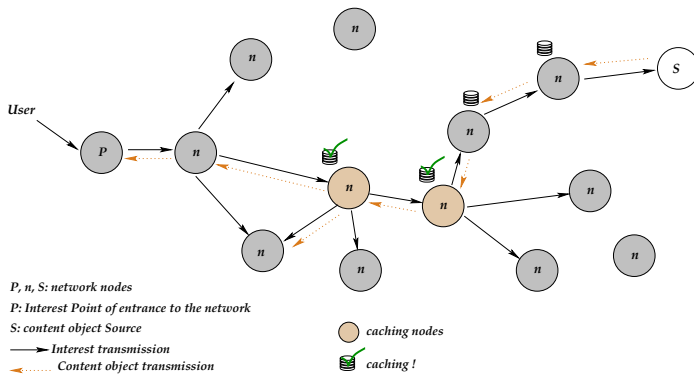
Figure 5: An example of function of our strategy when \Delta is equal to 50% and x > 3 .
