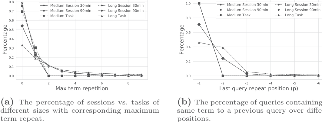
Fig. 3. Term repetition trends over sessions vs. tasks.
