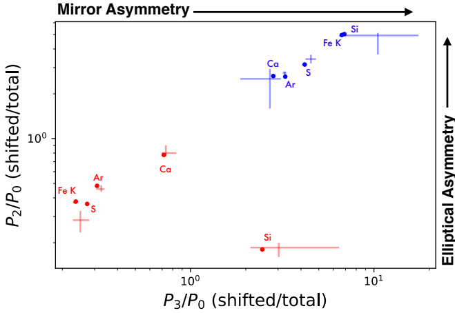
Fig. 5: The quadrupole power-ratios P_2/P_0 versus the octupole power-ratios P_3/P_0 of the red- and blue-shifted images of the different line emissions shown in Fig. 3, normalized with the quadrupole and octupole power-ratios of the total images. The dots and errorbar as obtained in the same way as in Fig. 4
