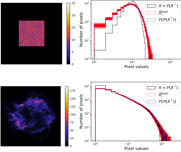
Fig. B.2: Data sets and their associated histogram in two cases : on top, the very simple case of a Poisson realization of the image of a square with uniform value 10 ; on the bottom, a toy model Cas A image obtained by taking a Poisson realization of a high-statistics denoised image of Cas A (hereafter called toy model). On the right, the black histogram correspond to the original data X = P(X^*) . The red histograms are those of the data sets \tilde{X}^{boot} obtained through resampling of the original data and the blue ones are the histograms of a Poisson realization of the original data P(X) = P(P(X^*)) . It appears that the resampled data sets have histograms highly similar to that of the original data with additional Poisson noise.
