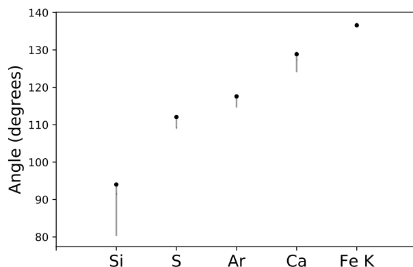
Fig. 7: Angles between the directions of the red- and blue-shifted centers of emission toward the center of explosion for each element.
