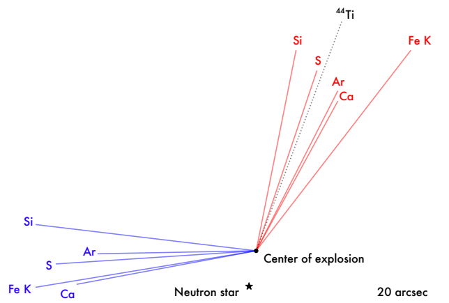
Fig. 6: Centroids of the blue- and red-shifted parts of each line emission and their distance from the center of explosion of Cas A. For reference, we added the direction of motion of the ^{44}\text{Ti} in black, as shown in Fig. 13 of Grefenstette et al. (2017). Only the direction is relevant, as the norm of this specific vector is arbitrary.
