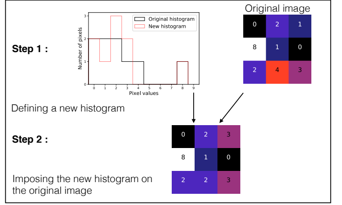
Fig. B.4: Scheme resuming the two steps of our new constrained bootstrap method.
