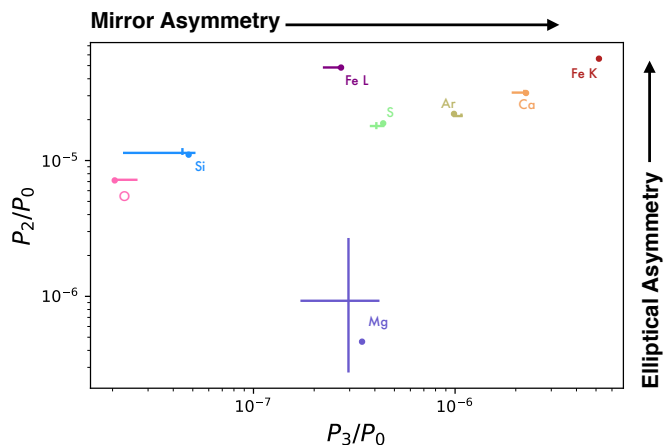
Fig. 4: The quadrupole power-ratios P_2/P_0 versus the octupole power-ratios P_3/P_0 of the total images of the different line emissions shown in Fig. 2. The dots represent the values measured for the pGMCA images obtained from the real data, and the crosses the 10 th and 90 th percentiles obtained with pGMCA on a hundred constrained bootstrap resamplings, with the center of the cross being the median.
