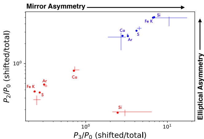
Fig. 5: The quadrupole power-ratios P_2/P_0 versus the octupole power-ratios P_3/P_0 of the red- and blue-shifted images of the different line emissions shown in Fig. 3, normalized with the quadrupole and octupole power-ratios of the total images. The dots and errorbar as obtained in the same way as in Fig. 4
