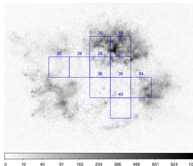
Fig. 9: Counts image of the Fe-K red-shifted component overlaid with the extraction regions used for the ^{44}\text{Ti} NuSTAR study of Grefenstette et al. (2017). The regions 19 and 20 which dominate our image in terms of flux have respective velocities moving away from the observer of 2300 \pm 1400 and 3200 \pm 500 \text{ km sec}^{-1} .
