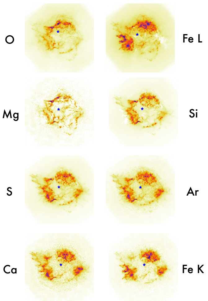
Fig. 2: Total images of the different line emissions' spatial structure as retrieved by the pGMCA. The blue dot represents the image centroid adopted in the PRM analysis. The color-scale is in square root.
