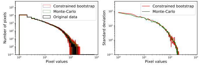
Fig. B.5: On the left, histogram of the original data, the resampled data sets and the MC realizations of the toy model Cas A image. On the right, the standard deviations of the resampled data sets and MC realizations bin by bin of the histogram on the left. We can notice the great adequation between the standard deviations of the resampled data sets and that of the MC realizations.
