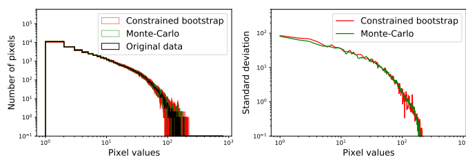
Fig. B.5: On the left, histogram of the original data, the resampled data sets and the MC realizations of the toy model Cas A image. On the right, the standard deviations of the resampled data sets and MC realizations bin by bin of the histogram on the left. We can notice the great adequation between the standard deviations of the resampled data sets and that of the MC realizations.
