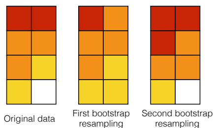
Fig. B.1: An example of bootstrap resampling. Each square represents a different event, each color a different value. N events are taken randomly with replacement from the original data to create each of the two bootstrap resamplings.
