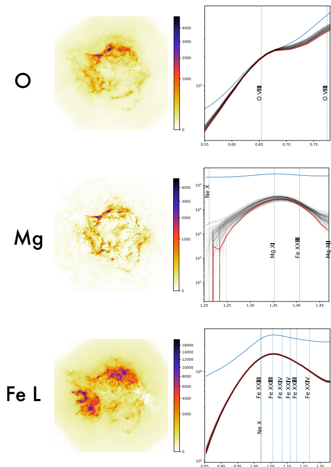
Fig. 8: Images of the O, Mg, and Fe L line emission spatial structures and their associated spectrum as found by pGMCA. The spectra in red correspond to the application of the algorithm on real data, while the dotted gray spectra correspond to the application on a hundred constrained bootstrap resamplings.
