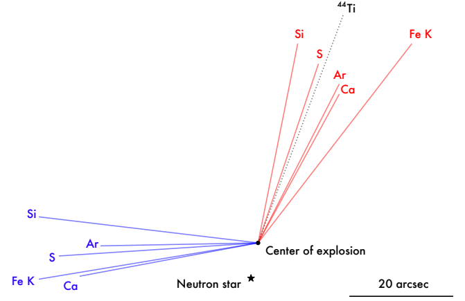
Fig. 6: Centroids of the blue- and red-shifted parts of each line emission and their distance from the center of explosion of Cas A. For reference, we added the direction of motion of the ^{44}\text{Ti} in black, as shown in Fig. 13 of Grefenstette et al. (2017). Only the direction is relevant, as the norm of this specific vector is arbitrary.
