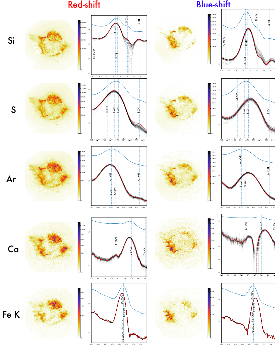
Fig. 3: Red- and blue-shifted parts of the Si, S, Ar, Ca and Fe line emission spatial distribution and their associated spectrum as found by pGMCA. The spectra in red correspond to the application of the algorithm on real data, while the dotted gray spectra correspond to the application on a hundred constrained bootstrap resamplings. The dotted lines represent the energy of the brightest emission lines for a non-equilibrium ionization plasma at a temperature of 1.5 keV and ionization timescale of \log(\tau) = 11.3 \text{ cm}^{-3} \text{ s} produced using the AtomDB (Foster et al. 2012). These parameters are the mean value of the distribution shown in Fig.2 of Hwang & Laming (2012).
