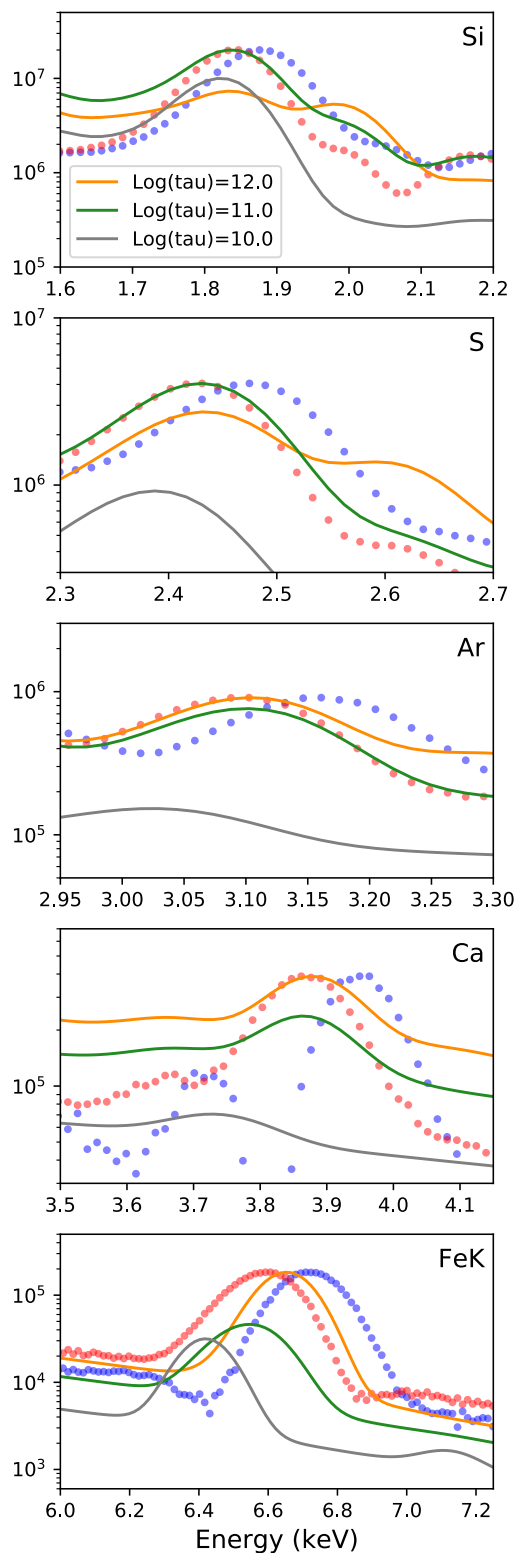
Fig. A.1: Comparison of our red/blue spectra (dotted curves) presented in Fig. 3 versus pshock Xspec models with different ionization timescales for kT=1.5 keV.
