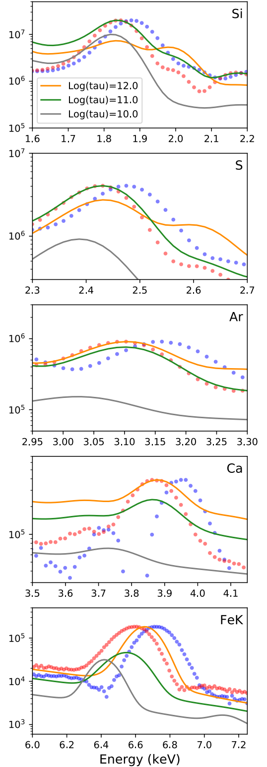
Fig. A.1: Comparison of our red/blue spectra (dotted curves) presented in Fig. 3 versus pshock Xspec models with different ionization timescales for kT=1.5 \text{ keV} .
