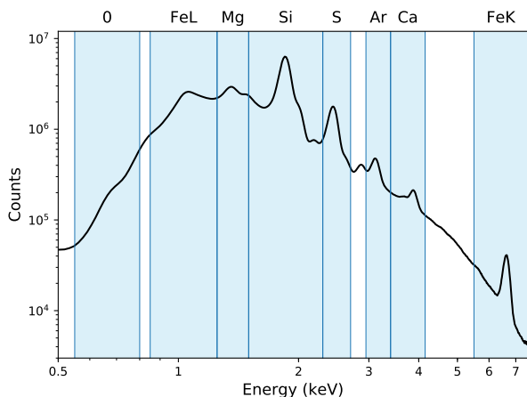
Fig. 1: Spectrum of Cas A obtained from the combination of the deep Chandra 2004 observations. The source separation algorithm was applied in each individual energy band represented by the shaded regions.
