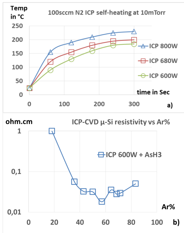
Figure 2. a) Thermal calibration for special substrate holder using 100sccm N 2 ICP at 10mTorr. b) Impact of Ar dilution in the ICP-CVD mixture (SiH 4 /H 2 /Ar/AsH 3 ) on \mu -Si resistivity at 4mTorr. Deposition is achieved on oxidized wafer.
