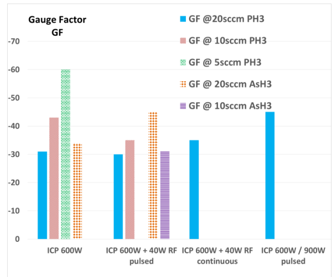
Figure 12. GF according to different ICP-CVD conditions.
