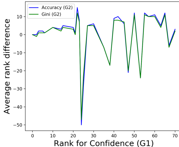
Fig. 6. Rank correlations
