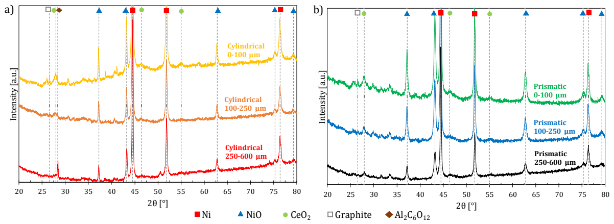
Figure SI-2 Powder XRD analysis of the 0-100 μm, 100-250 μm and 250-600 μm fraction for the (a) cylindrical-type type batteries and (b) prismatic-type batteries
