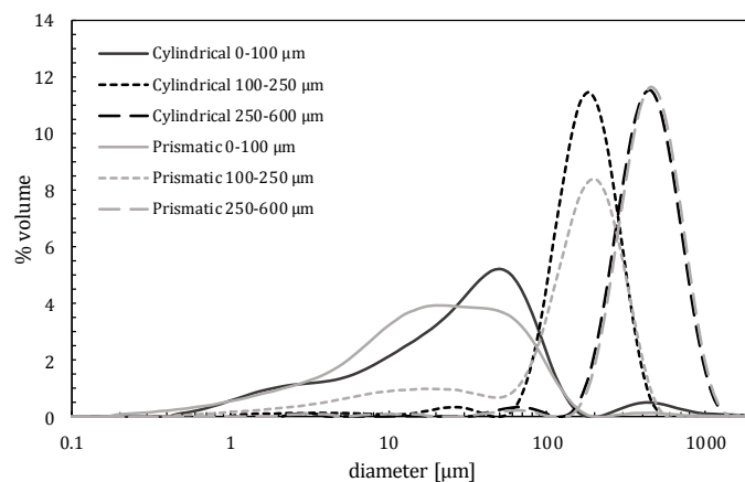
Figure SI-1 Particle size distribution [%vol] of the 0-100 \mu\text{m} , 100-250 \mu\text{m} and 250-600 \mu\text{m} fractions obtained from the cylindrical-type and prismatic-type batteries
