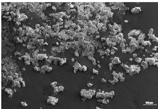
Figure 3: Scanning Electron Microscope observation of detached grains of a "non-sensitized" 304L SS [8].
