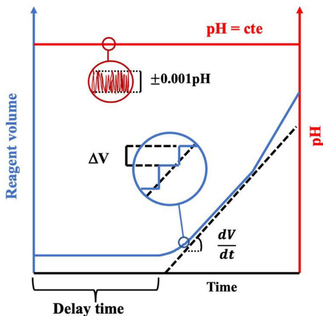
Fig. 2. Typical curve of constant composition crystallization experiment. The step in the volume curve ( \Delta V ) corresponds to the volume resolution of the burette, \Delta \text{pH} = 0.001 corresponds to the resolution of the pH probe. The time between two pH oscillations corresponds to the time resolution of the experiment. The typical blue curve consists of an initial plateau, characteristic of the delay time and of an increase of the volume added corresponding to crystal growth. In some cases, a change of the injected volume is observed and is characteristic of a change in the crystallization mechanism (growth, nucleation or different phase crystallization).
