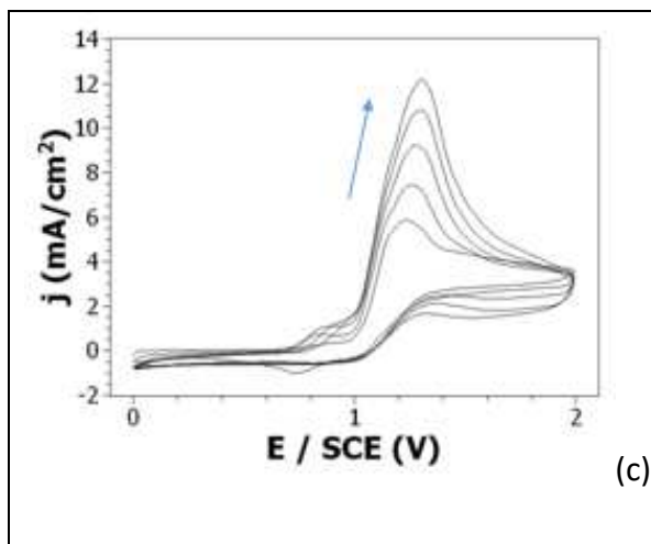
Figure 5: Cyclic voltammograms at a Pt electrode obtained in a: (a) Cz:CzE 95:5, (b) Cz:CzE 90:10, (c) Cz:CzE 70:30 acetonitrile + 0.1 M LiClO 4 solution. Scan rate of 50 mV/s.
