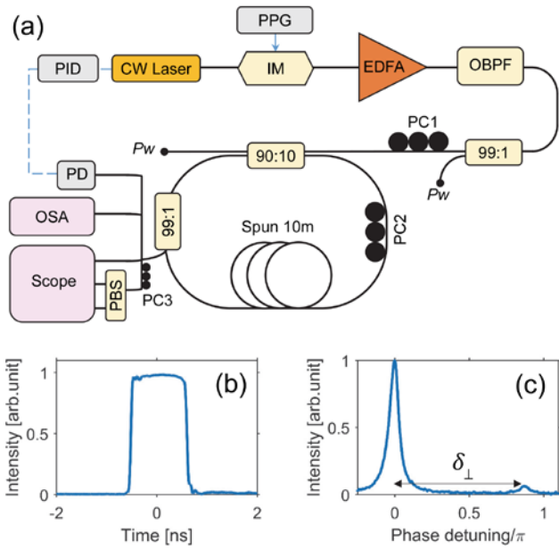
Fig. 1. (a) Experimental setup. PPG: pulse pattern generator, IM: intensity modulator, PC: polarization controller, EDFA: erbium doped fiber amplifier, OBPF: optical bandpass filter, PBS: polarization beam splitter, OSA: optical spectrum analyzer, PID: proportional integral derivative system, PD: photodetector, PW: power-meter. (b) Input pulse profile. (c) Linear resonances of the cavity.
