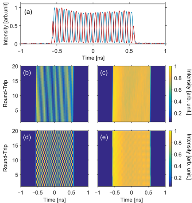
Fig. 4. (a) Typical experimentally measured temporal intensity profiles of both orthogonal polarization components (at 45^\circ with respect to the driving and PMI sidebands SOPs) monitored at the output of the cavity for \delta_\perp slightly positive (low PMI frequency, within the bandwidth of our detectors). (b) Round-trip by round-trip evolution (from bottom to top) of the temporal intensity profile at the output of our fiber cavity monitored on one of the polarization components (as used in panel (a)) for \delta_\perp slightly above 0. (c) Corresponding total intensity (before the PBS). (d, e) Same as (b, c) but with \delta_\perp slightly above -\pi .
