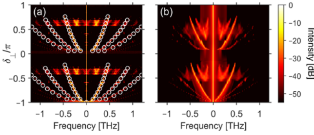
Fig. 2. Pseudo-color plots of (a) numerical and (b) experimental output spectra for various values of relative detuning \delta_{\perp} , i.e., intra-cavity birefringence. Circles in (a) highlight how the position of the PMI sidebands match the theoretical predictions of Eq. (4). Driving power X=28 and linear detuning \Delta=8 . Spectra are plotted as a function of frequency detuning from the central cw driving component.
