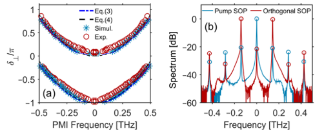
Fig. 3. (a) Optimum frequency ( \Omega_{\text{opt}} ) of the first-order PMI sidebands versus relative detuning \delta_{\perp} . Experimental results (red circles) are compared with numerical simulations (blue stars) as well as theoretical predictions of Eqs. (3)–(4) (blue and black dashed-lines, respectively). (b) Output spectrum for \delta_{\perp} = 0.2\pi recorded after the output PBS and decomposed into polarization components parallel (blue) and orthogonal (red) to the driving SOP.
