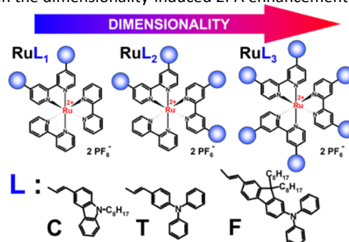
Scheme 1. Molecular structures of the Ru-complexes.
