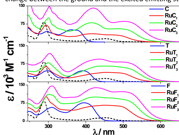
Fig.1 Absorption spectra (full lines) of the ligands and their corresponding Ru-complexes in THF. Dashed lines: Absorption spectrum of Ru(bpy) 3 2+ in acetonitrile.
