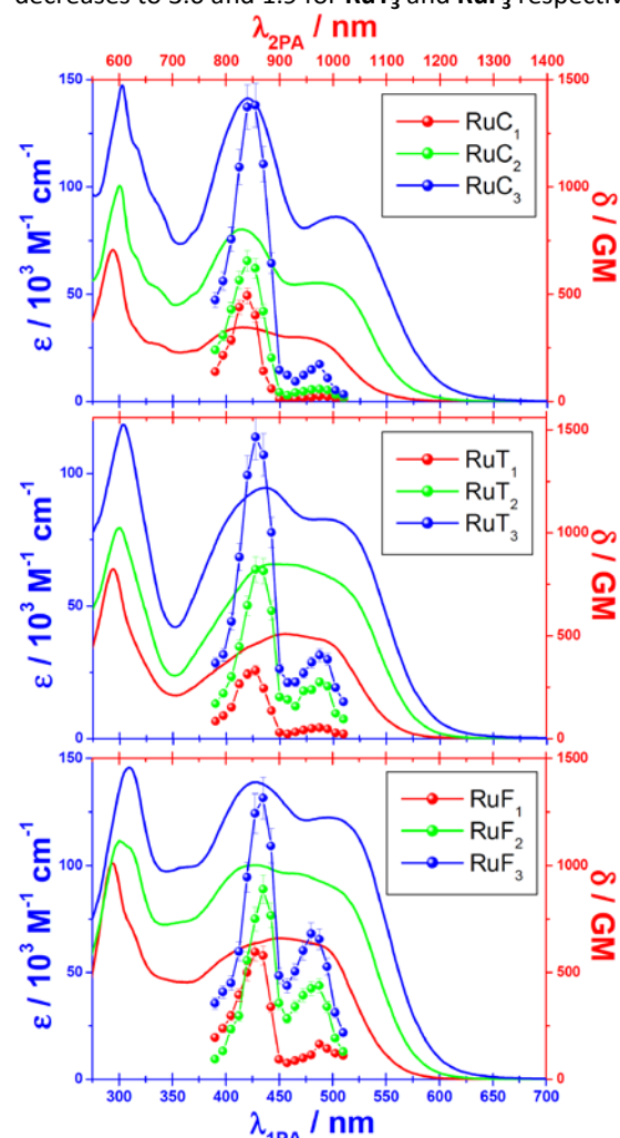
Fig.2 1PA (full lines) and 2PA (symbols) spectra of Ru-complexes in THF. The one-photon molar absorption is shown at the 1PA wavelength (lower horizontal scale). The 2PA cross section is shown as a function of the excitation laser wavelength (upper horizontal scale).
