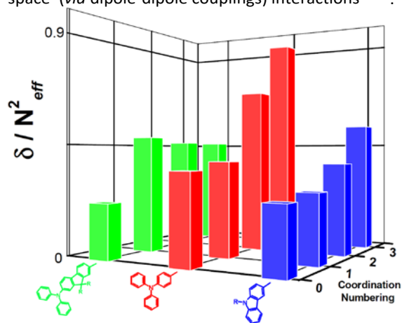
Fig.3 Intrinsic 2PA performance of all the dyes as function of ligands \pi -conjugation length and complexes coordination number.
