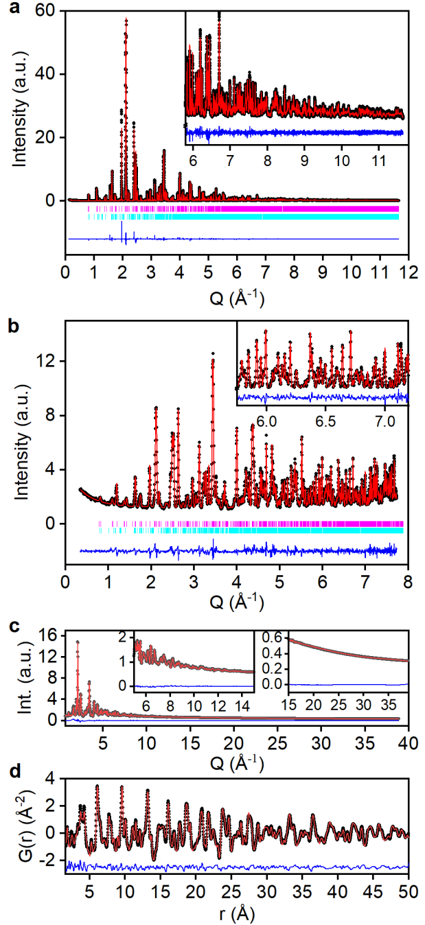
Figure 1. Structural refinements of \text{La}_2\text{Ga}_3\text{O}_{7.5} in Im2 . (a,b) Combined Rietveld refinement against SPD data from 11BM, and NPD data from D2B, with the fits to the high- Q regions inset. (c,d) Simultaneous Rietveld and PDF fit against SPD data from I15-1. Magenta ticks = \text{La}_2\text{Ga}_3\text{O}_{7.5} , cyan ticks = \text{La}_4\text{Ga}_2\text{O}_9 (~2wt%). Black points = y_{\text{obs}} , red line = y_{\text{calc}} , blue line = y_{\text{obs}} - y_{\text{calc}} .
