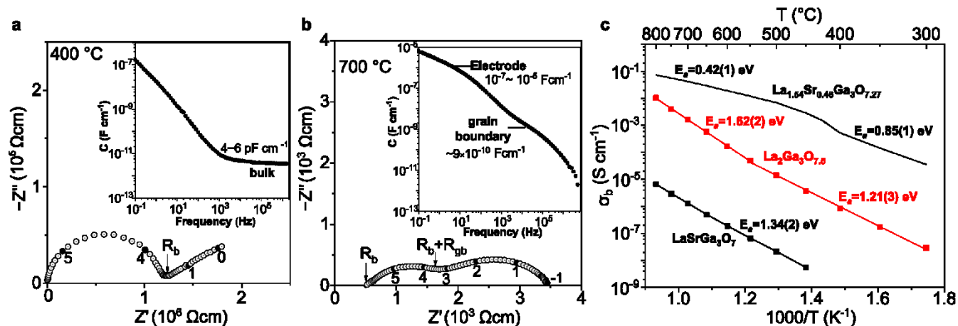
Figure 6. Complex impedance plots at (a) 400^\circ\text{C} and 700^\circ\text{C} of the \text{La}_2\text{Ga}_3\text{O}_{7.5} ceramic. R_b and R_b+R_{gb} denote the bulk and total resistivities, respectively. The inset in each part shows capacitance versus frequency plot. (c) Arrhenius plot of the bulk conductivities for \text{La}_2\text{Ga}_3\text{O}_{7.5} (red points) in comparison with those of \text{LaSrGa}_3\text{O}_7 (black points) and \text{La}_{1.54}\text{Sr}_{0.46}\text{Ga}_3\text{O}_{7.25} (black line, data from reference 14).
