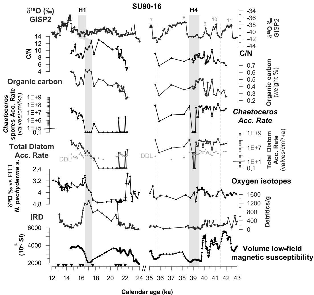
Figure 5. Core SU90-16: volume low-field magnetic susceptibility \kappa ( 10^{-6} SI); IRD \text{g}^{-1} ; \delta^{18}\text{O} N. pachyderma s. versus PDB; diatom accumulation rate (valves \text{cm}^{-2} \text{ka}^{-1} ) (taken as proxy for productivity); Chaetoceros spores accumulation rate (valves \text{cm}^{-2} \text{ka}^{-1} ) (taken as spring bloom indicator); organic carbon (wt %); C/N ratio for HE 1 and HE 4 time slices. Triangles on the age axis stand for radiocarbon dates.
