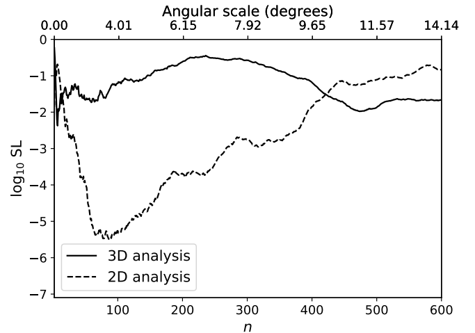
Fig. 8. Logarithm of the significance level at which position angle uniformity should be rejected as a function of the number of nearest neighbors n for the 1051 sources with total flux density >108 mJy and a redshift measurement. The dashed line indicates the results of the 2D analysis and the solid line the results of the 3D analysis.
