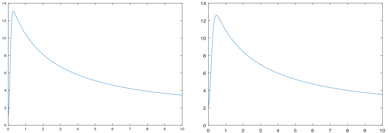
FIGURE 3. Left: \sigma = 1.4 , \theta = -0.01 , \vartheta = 1 with H_{DP}(0) = 0.98 , H_{DP}(\infty) = 2.5544 , Right: \sigma = 2 , \theta = -0.01 , \vartheta = 1 with H_{DP}(0) = 2 , H_{DP}(\infty) = 2.5821 .
