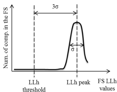
Fig. 1 GTM Applicability Domain is identified by log likelihood threshold LLh_0 = LLh_{peak} - 3\sigma . Here, LLh_{peak} and \sigma are, respectively, a position and with of a Gaussian function which fits the LLh distribution
