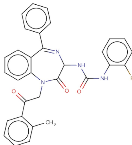
AMS structure ID 414778192 Target: Cholecystikinin B receptor Probability to be active is 92%
