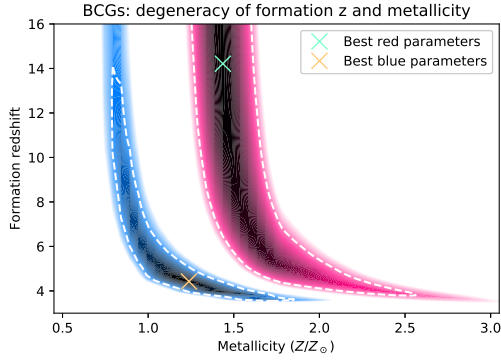
Fig. 11. Contour plots for the red and blue BCG sub-samples showing the \chi^2_v value as a function of the two varying parameters (formation redshift and metallicity). Dashed white curves correspond to the 68% confidence limit. The coloured regions correspond to the 95% confidence interval. The tested metallicity range is Z = 0.1 Z_\odot to Z = 5 Z_\odot , but here it is restricted to Z = 0.5 Z_\odot to Z = 3.5 Z_\odot . The tested formation redshift range is z_{\text{form}} = 3 to z_{\text{form}} = 16 . The cross displays the location of the best fit parameters.
