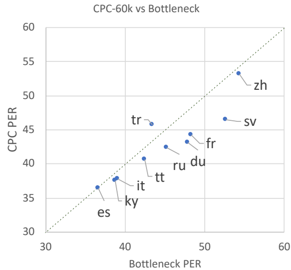
Fig. S1. CPC versus Bottleneck features. The CPC features here have been trained on the 60Kh libri-light dataset.
