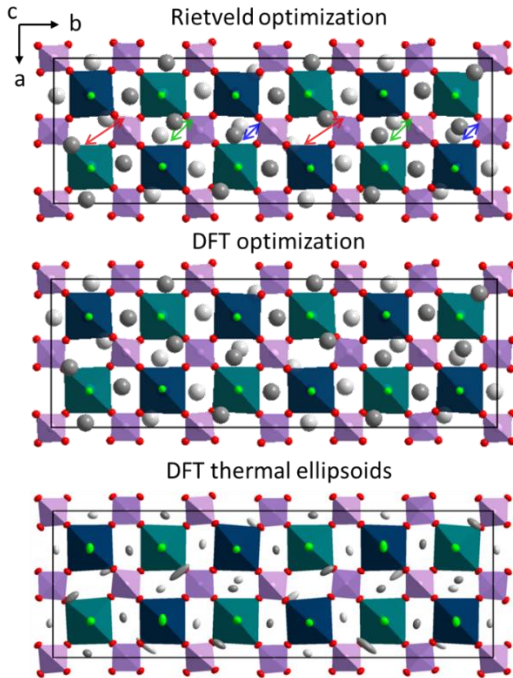
Figure 8. Polyhedral representation of optimal A2_1am structure of LT-NVPF obtained after Rietveld refinement (top) and after DFT structure relaxation (center). The large (red), medium (blue), and small (green) gaps between Na ions in the center row are indicated by arrows. An additional plot of the second DFT calculation used to obtain atomic displacement parameters is also shown (bottom) with the thermal ellipsoids drawn at the 90% level. The VO_6 octahedra are shown in dark blue when the apical F is in the Na plane and in teal otherwise, and the PO_4 tetrahedra are shown in mauve. Na atoms are shown in dark grey in the upper layer and light grey in the lower layer, O are shown in red, and F in green.
