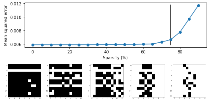
Figure 6: Top: MSE of the prediction. Black line is the sparsity of the inferred causal graph. Bottom: Causal graphs for different sparsity levels. Fourth image is the inferred causal graph.
