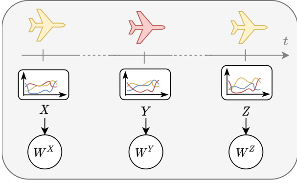
Figure 2: Under the assumption that a unique causal graph \mathcal{G} represents the causal structure underlying a mechanical system (here a plane), we claim that, if the causality assumption is relevant, the respective set of edge’s weights W^X , W^Y and W^Z associated to the MTS samples X , Y and Z can characterize the state of the system. Here, following the color code, W^Z should be closer from W^X than from W^Y . We note that a maintenance was effectuated between Y and Z to restore the system’s state.
