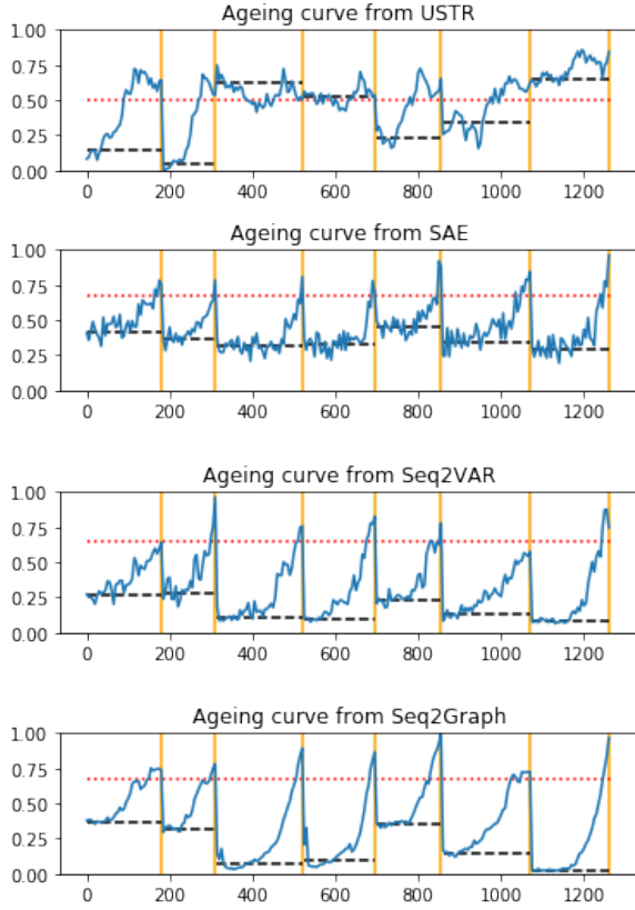
Figure 7: Unsupervised estimation of C-MAPSS ageing curve with different models on the 7 first test batches. From top to bottom: USTR [9], SAE [17], Seq2VAR [22], Seq2Graph. Orange picks are engine failures and repair. Long red dotted horizontal line is the threshold \tau^{valid} . Black dashed horizontal lines are the estimated initial states of each engine, computed as the mean value of the curve on the 10 first samples of each batch.
