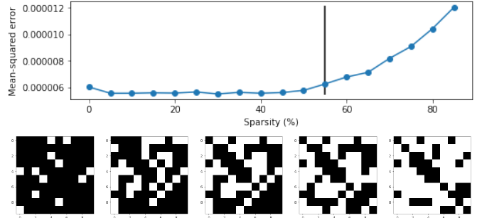
Figure 4: Top : Prediction MSE. Black line is the true sparsity. Bottom : Causal graphs for different sparsity levels. The third figure is the inferred causal graph, which matches the ground truth.
