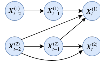
Figure 1: Graphical representation of the causality underlying a bivariate time series X . The edges are weighted with a set of edge’s weights W^X that depends on X . In this paper, we claim that comparing MTS samples by comparing their causality weights is relevant.
