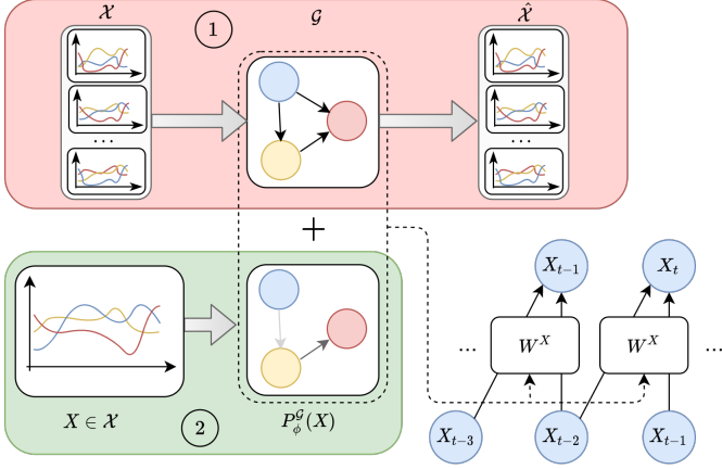
Figure 3: Seq2Graph. ① is the dataset-level causal graph \mathcal{G} inference. \hat{\mathcal{X}} is the set of predictions for the whole dataset \mathcal{X} . \mathcal{G} is built such that it explains the mean dynamical behavior of the dataset. ② is the representation inference. \hat{X} is the prediction of the sample X . The adjustments P_\phi^{\mathcal{G}}(X) are built such that they explain the specific causality underlying sample X , along the edge of the mean parameter \bar{W} . Here, K = 2 .
