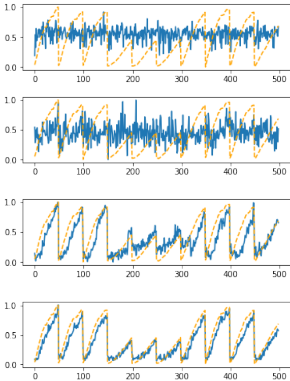
Figure 5: Unsupervised estimation of ageing curves for the 10 first batches of the test set. From top to bottom: USTR [9], SAE [17], Seq2VAR [22], Seq2Graph. Orange curve is the ground truth.
