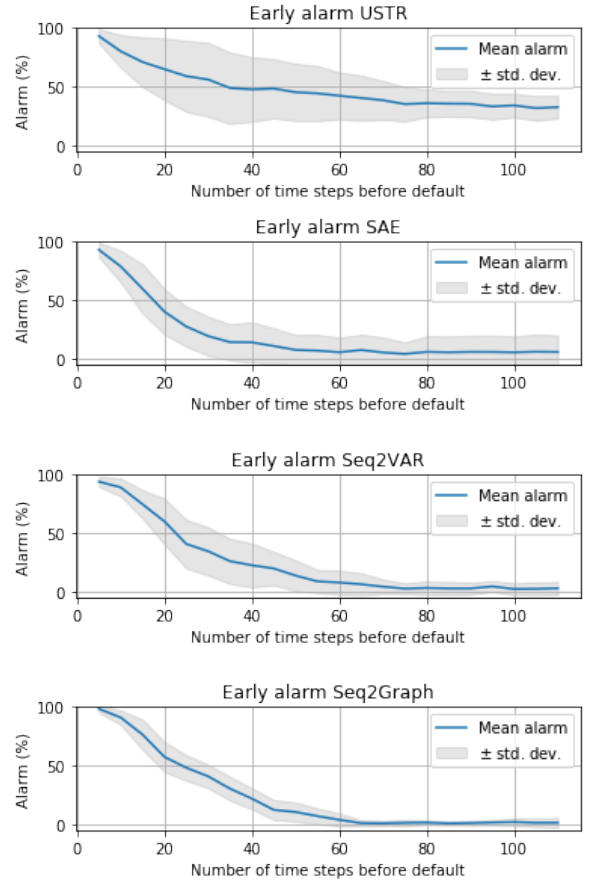
Figure 8: Early alarm on CMAPSS data using MTS representation models USTR, SAE, Seq2VAR (see related work for details) and Seq2Graph. Means and standard deviations are built using all batch’s first samples as X^{ref} and several encoders trained with different seeds.
