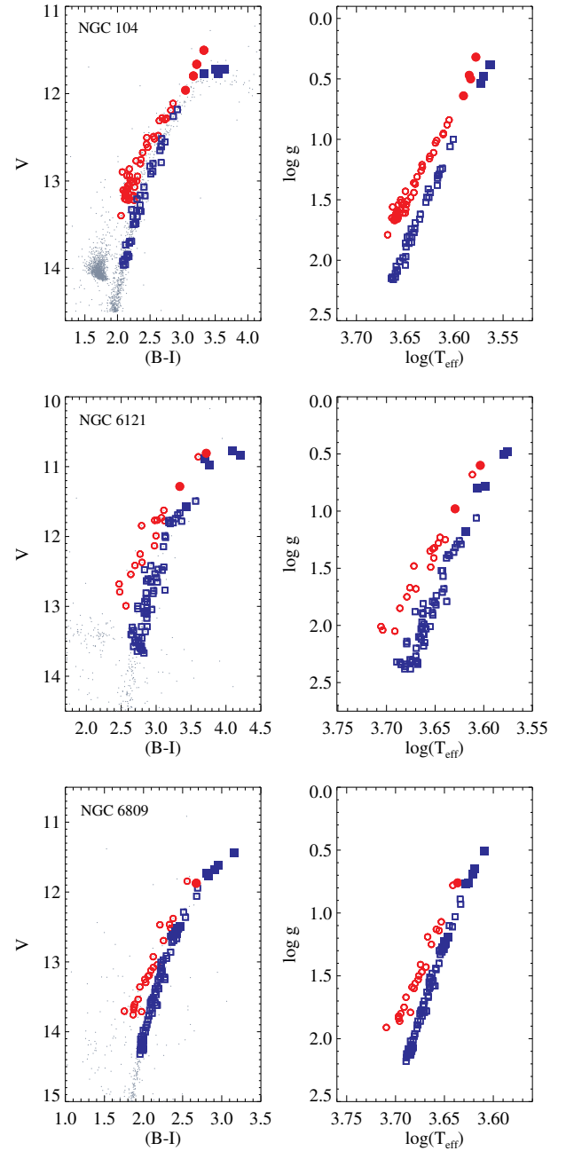
Fig. 1. Photometric CMDs ( left ) and \log g - \log T_{\text{eff}} distributions ( right ) of the cluster member stars. Red circles and blue squares represent AGB and RGB stars, respectively, while the GIRAFFE and UVES samples can be distinguished by open and filled symbols, respectively. The same symbols are used throughout the paper.
