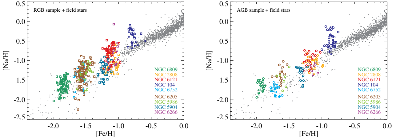
Fig. 9. [\text{Na}/\text{H}] (NLTE) as a function of [\text{Fe}/\text{H}] for RGB ( left ) and AGB ( right ) stars in the nine GCs discussed in this paper (our analysis for NGC 104, NGC 2808, NGC 6121, NGC 6809, and NGC 6752; literature data for NGC 5904, NGC 5986, NGC 6205, and NGC 6266) and in Galactic field stars from Carretta (2013, gray points).
