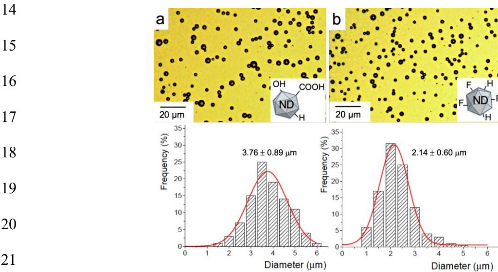
22 Figure 3. Optical micrographs of F -hexane-stabilized microbubbles shelled with a) ND25 and b) 23 F -ND25, with corresponding size distributions. Concentration: 0.1 \text{ g L}^{-1} ; pH 12.0.
