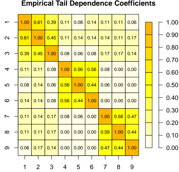
Figure 3: The empirical pairwise tail dependence coefficients \widehat{\chi}_{ij}(u_i, u_j) , 1 \leq i, j \leq 9 based on the empirical 95%-quantiles as thresholds. Here stations 1–3 belong to the region in the northwest, stations 4–6 to the region in the south and stations 7–9 to the region in the northeast of France.
