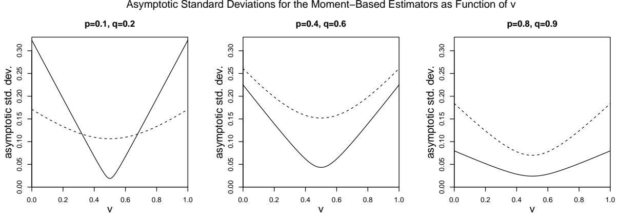
Figure 1: The asymptotic standard deviations \sqrt{V((v, 1-v))} (solid lines) and \sqrt{\tilde{V}((v, 1-v))} (dashed line) of the moment-based estimators with known and unknown margins, respectively, for each of the three scenarios reflecting strong, moderate and weak dependence (from left to right).
