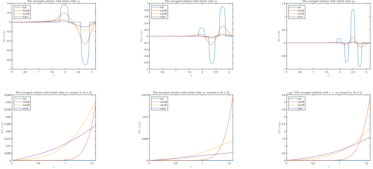
Figure 1: The averaged solutions of the heat equation when G = (0, \pi) , G_0 = (0, \pi/2) , \rho = 1_{(0,1)} with initial values of the sequence given in the proof of Proposition (see (A.1)) and with \varsigma given by (5.5).
