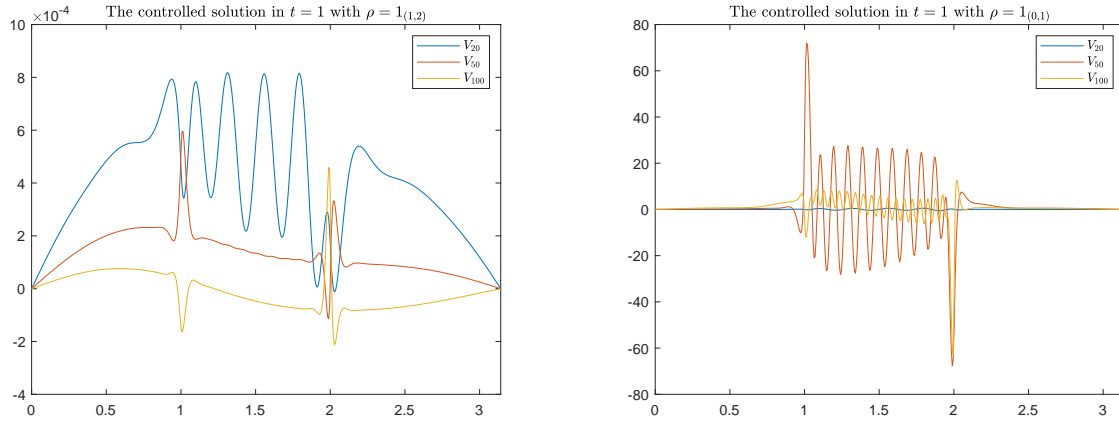
Figure 4: The state at time t = 1 of the averaged solutions of the heat equation after applying the function induced by the minimum of J in V_{20} , V_{50} and V_{100} with y^0 = \frac{1}{2} . In the left figure we have considered \rho = 1_{(1,2)} and we observe that those functions are controls that take the solutions almost to equilibrium. The computations are obtained by approximating the density functions with Dirac masses, which explains why the solution does not converge exactly to 0. In the right one, \rho = 1_{(0,1)} and we see that the minimum of J do not take the solutions to equilibrium, so the functions that we have obtained cannot be considered controls.
