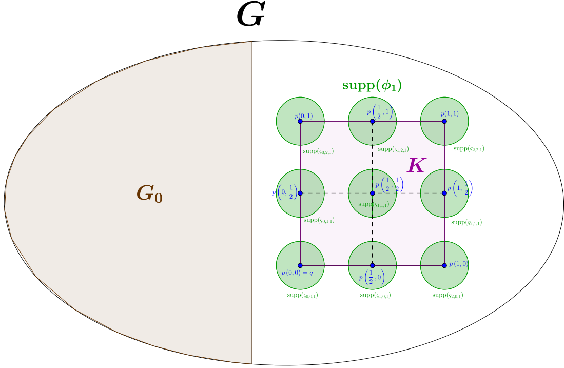
Figure 5: An illustration of the support of \phi_1 in a domain belonging to \mathbb{R}^2 .
