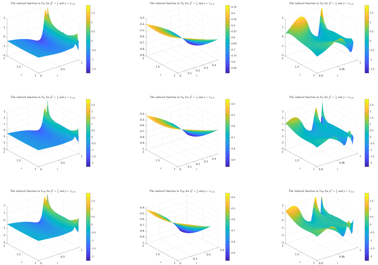
Figure 2: Graphs of the functions for \rho = 1_{(1,2)} and y^0 = \frac{1}{2} induced by the minimum of the functional J in V_{20} , V_{50} and V_{100} . In the left column we illustrate the whole graphs, in the middle column we illustrate the graphs with the time variable zoomed in [0, 1/2] , and in the right column zoomed in [0.9, 1] .
