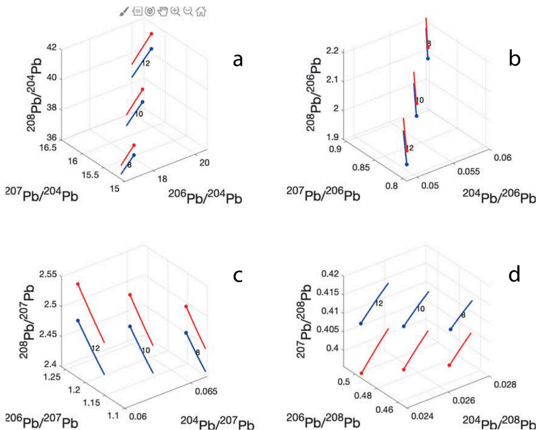
Fig. 1. The four possible ternary plots involving ratios with the same reference (denominator) isotope showing how Pb isotope ratios evolve through time as a function of the tectonic, or geological, ‘model’ age T_m and the \mu ( ^{238}\text{U}/^{204}\text{Pb} \propto \text{U}/\text{Pb} ) and \kappa ( ^{232}\text{Th}/^{238}\text{U} \propto \text{Th}/\text{U} ) parameters. Panels (a) to (d) correspond to normalization to ^{204}\text{Pb} , ^{206}\text{Pb} , ^{207}\text{Pb} , and ^{208}\text{Pb} , respectively. The blue and red stem-like segments correspond to evolution of the ratios with radiogenic ingrowth through geological time from 540 Ma ago to 0 (modern lead, represented as full circle symbols). The numbers labelling the lines indicate \mu values ( ^{238}\text{U}/^{204}\text{Pb} = 8, 10, 12 ). The blue and red colors indicate different \kappa values ( ^{232}\text{Th}/^{238}\text{U} = 3.8 and 4.2 , respectively). (For interpretation of the references to color in this figure legend, the reader is referred to the Web version of this article.)
