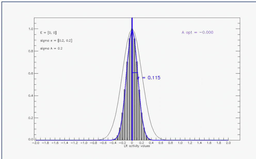
Figure 3: Comparison of the histogram and analytical probability distributions obtained for two pollutants. The known values of the total emissions E are set to 0 and the standard deviation of the original distributions of the LR activity and LR emission factors are set to 0.2. Both the histogram and analytical distributions are centered on the value of a_{opt} given by the theory. The original distribution of the LR activity is over plotted in black to indicate the precision gain between the original and constrained distributions.
