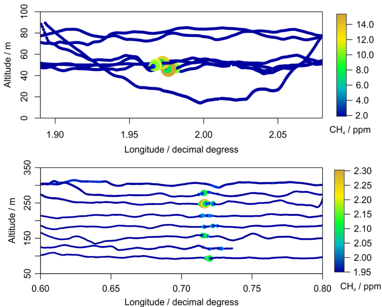
Figure 7. Plumes measured from separate installations to demonstrate the differences in strategies between 2018 and 2019. [upper panel] Plume sampled downwind with poorer vertical spatial resolution in the 2D plane during the 2018 portion of the campaign. CH 4 measured values are much higher due to platform activities during the survey time. [lower panel] Plume sampled downwind in 2019 with intermediate transects enabling higher vertical spatial resolution. Note the colour scale across each plot signifies different measured CH 4 ; the scales on the upper and lower plots are different.
