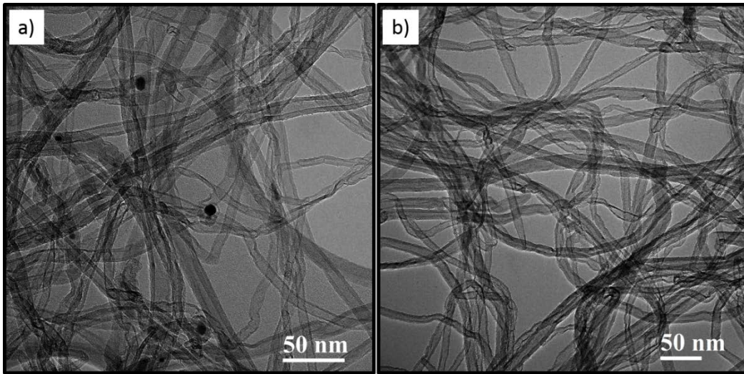
Figure 1. Typical TEM bright field micrographs of (a) rCNT and (b) pCNT with Cl 2 (at 1000°C for 2 h) followed by 2 h thermal treatment (1000°C) under nitrogen.
