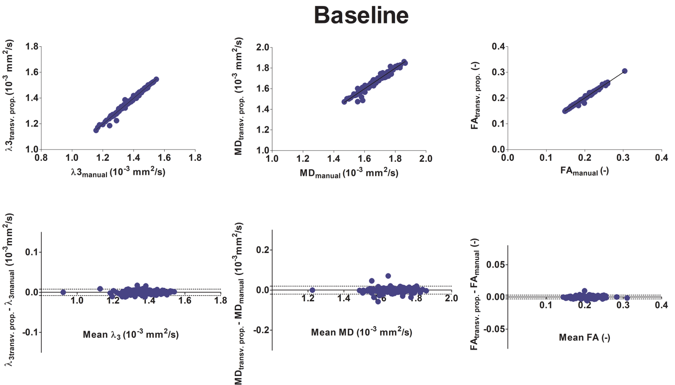
FIGURE 6 Linear regression analysis (top) and Bland-Altman plot (bottom) at baseline of diffusion indices \lambda_3 ( 10^{-3} mm 2 /s), MD ( 10^{-3} mm 2 /s) and FA (–) comparing manual segmentation with those resulting from the transversal propagations
