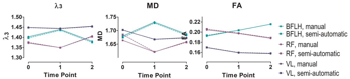
FIGURE 3 Comparison of the manual and semi-automatic segmentations of the mean values of \lambda_3 , MD and FA for the BFLH, RF and VL muscles of a representative subject at baseline, post-marathon and follow-up time points
