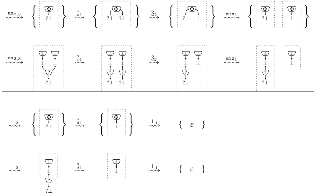
■ Figure 9 The path \text{Box}_2 \ ?_{d_1} \ \text{Box}_2 \ ?_{c_1} \ \text{Box}_2 \ ?_{d_2} \ \text{mix}_1 \ \perp_2 \ ?_{c_1} \ ?_{d_2} \ \text{mix}_1 \ \perp_2 \ ?_{d_1} \ \perp_1 witnessing that \rho \in \mathcal{T}(R) (continued from Figure 8).
