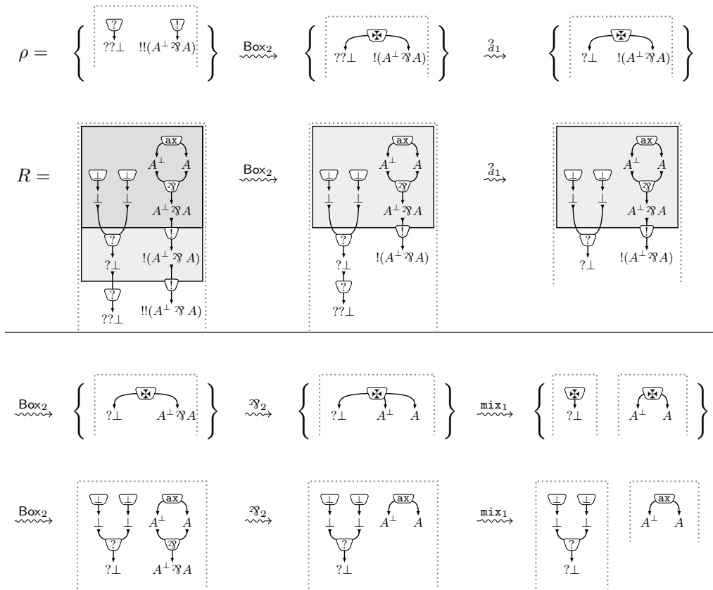
Figure 8 The path \text{Box}_2 \overset{?d_1}{\rightsquigarrow} \text{Box}_2 \overset{?d_2}{\rightsquigarrow} \text{mix}_1 \text{ax}_{2,3} \overset{?c_1}{\rightsquigarrow} \overset{?d_2}{\rightsquigarrow} \text{mix}_1 \perp_2 \overset{?d_1}{\rightsquigarrow} \perp_1 witnessing that \rho \in \mathcal{T}(R) (to be continued on Figure 9).
