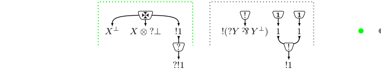
■ Figure 10 An element of the \eta -filled Taylor expansion of the MELL quasi-proof-structure in Fig. 2.
