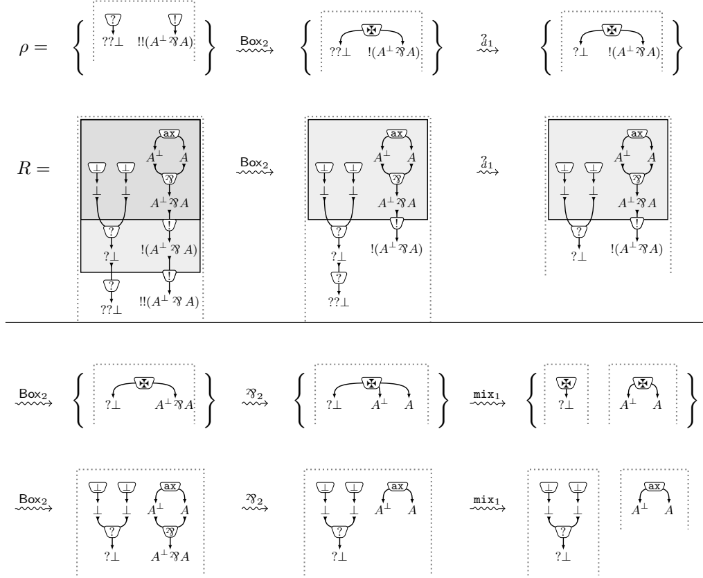
■ Figure 8 The path \text{Box}_2 \ ?_{d1} \ \text{Box}_2 \ ?_2 \ \text{mix}_1 \ \text{ax}_{2,3} \ ?_{c1} \ ?_{d2} \ \text{mix}_1 \ \perp_2 \ ?_{d1} \ \perp_1 witnessing that \rho \in \mathcal{T}(R) (to be continued on Figure 9).
