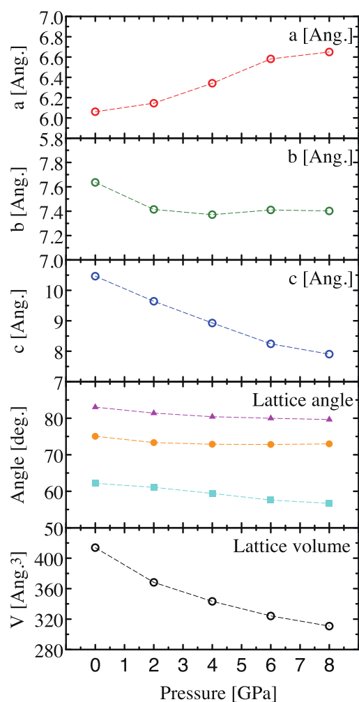
Fig. 11 Pressure dependence of DFT optimized lattice parameters in tricl -NiEt. The structural optimization is performed on the basis of exchange-correlation functional of vdW-DF2. Solid circles, triangles, and squares are lattice angles \alpha , \beta , and \gamma , respectively.
