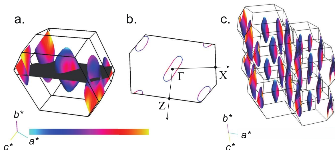
Fig. 10 Calculated Fermi surface of tricl-NiEt at 6 GPa. (a) First Brillouin zone; (b) 2D plane of the Fermi surface perpendicular to the b^* -axis containing the \Gamma -point, and (c) Bird's view of the Fermi surface of 2 \times 2 \times 2 cell of the first Brillouin zone. Color bar indicates Fermi velocity. The figures are plotted using FermiSurfer 2.1.0. 28
