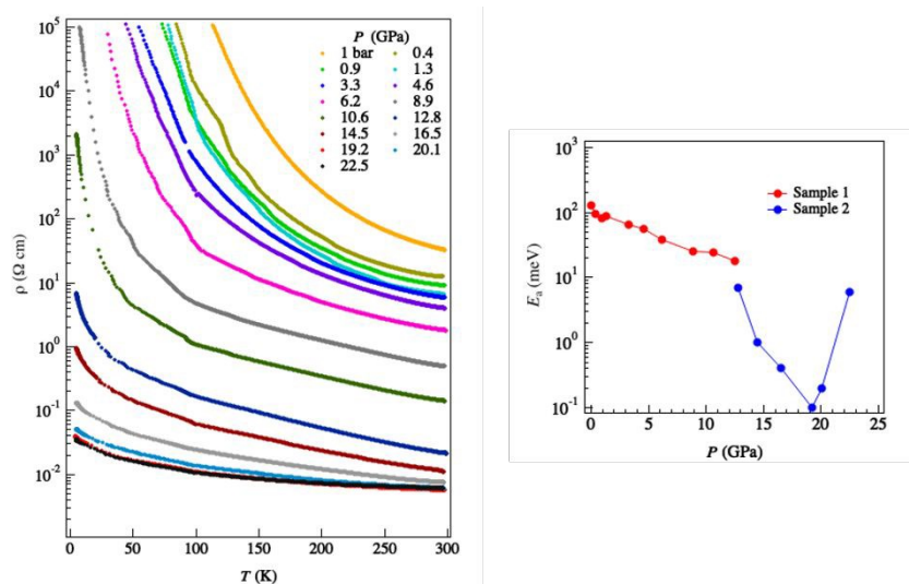
Fig. 6 Temperature dependence of the resistivity of NiMe as a function of temperature, and at different pressures between 1 bar and 22.5 GPa (left). Pressure dependence of the activation energy of NiMe (right).
