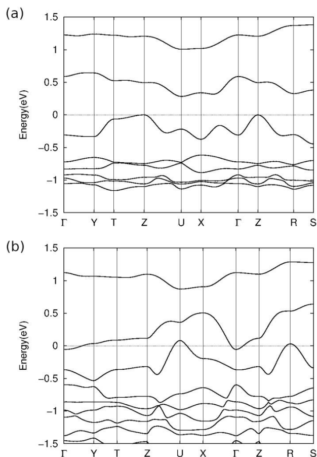
Fig. 9 First-principles band structure of tricl-NiEt at (a) ambient pressure and (b) 6 GPa. See Figure S6 for the calculated band structures at 2, 4 and 8 GPa and Figure S7 for details of the first Brillouin zone of the optimized structure of 6 GPa. The dotted lines at Energy = 0 eV in (a) and (b) represent the top of the valence bands and Fermi energy respectively.
