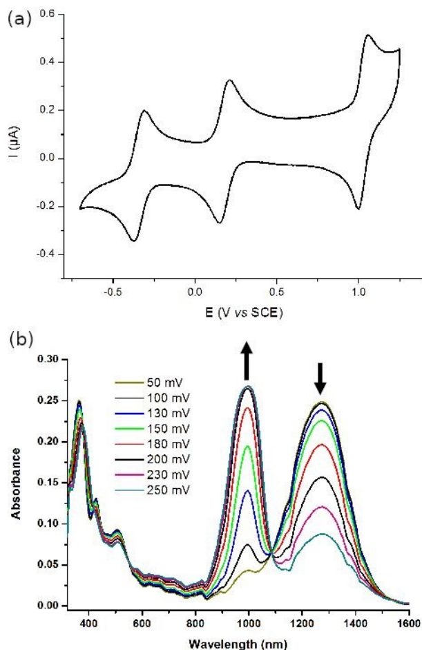
Fig. 1 (a) Cyclic voltammetry (b) and UV-Vis-NIR monitoring of the electrochemical oxidation of [\text{Bu}_4\text{N}][\text{Pt}(\text{Et-thiazdt})_2]
